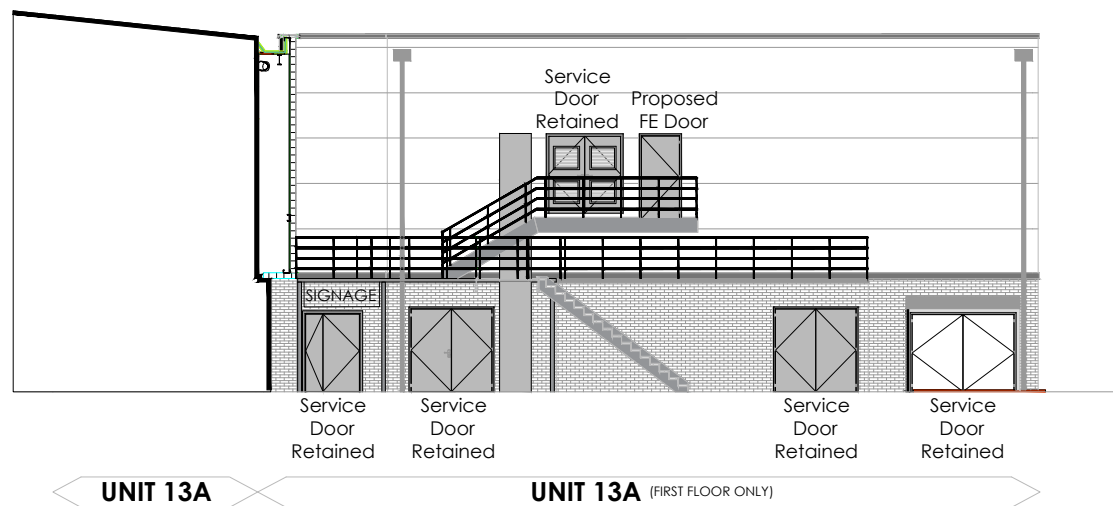
Elevation C - Rear
