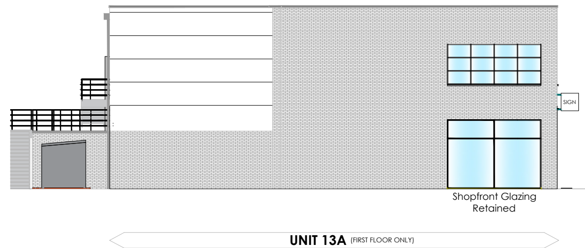
Elevation B - Facing F&B units
