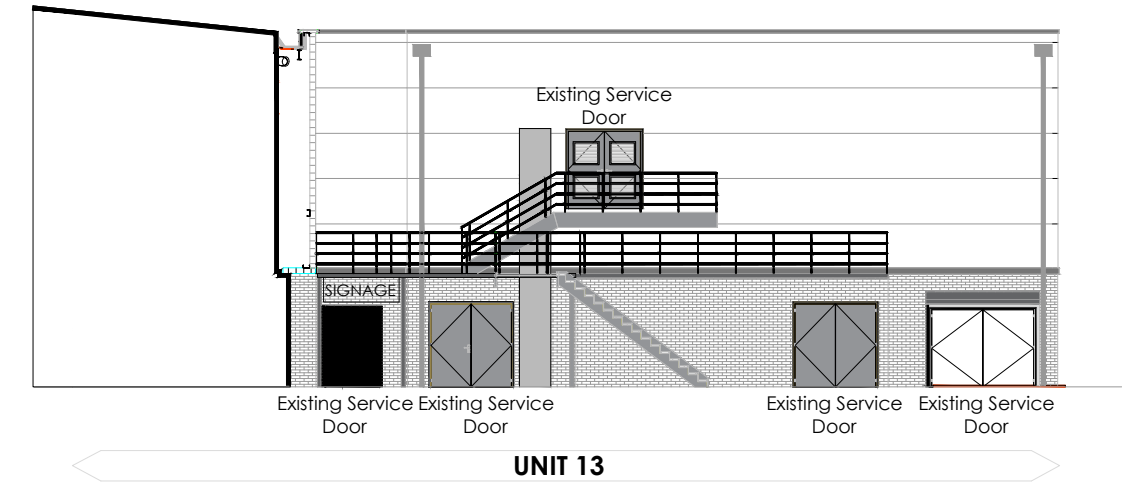
Elevation C - Rear
