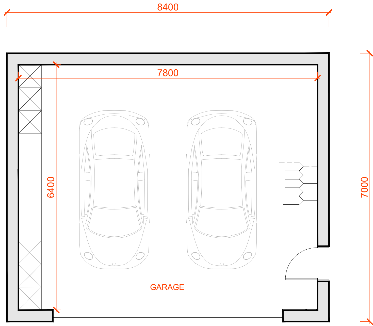
P1 Proposed Ground Plan (GIA 49.9sqm) 1:50@A1
