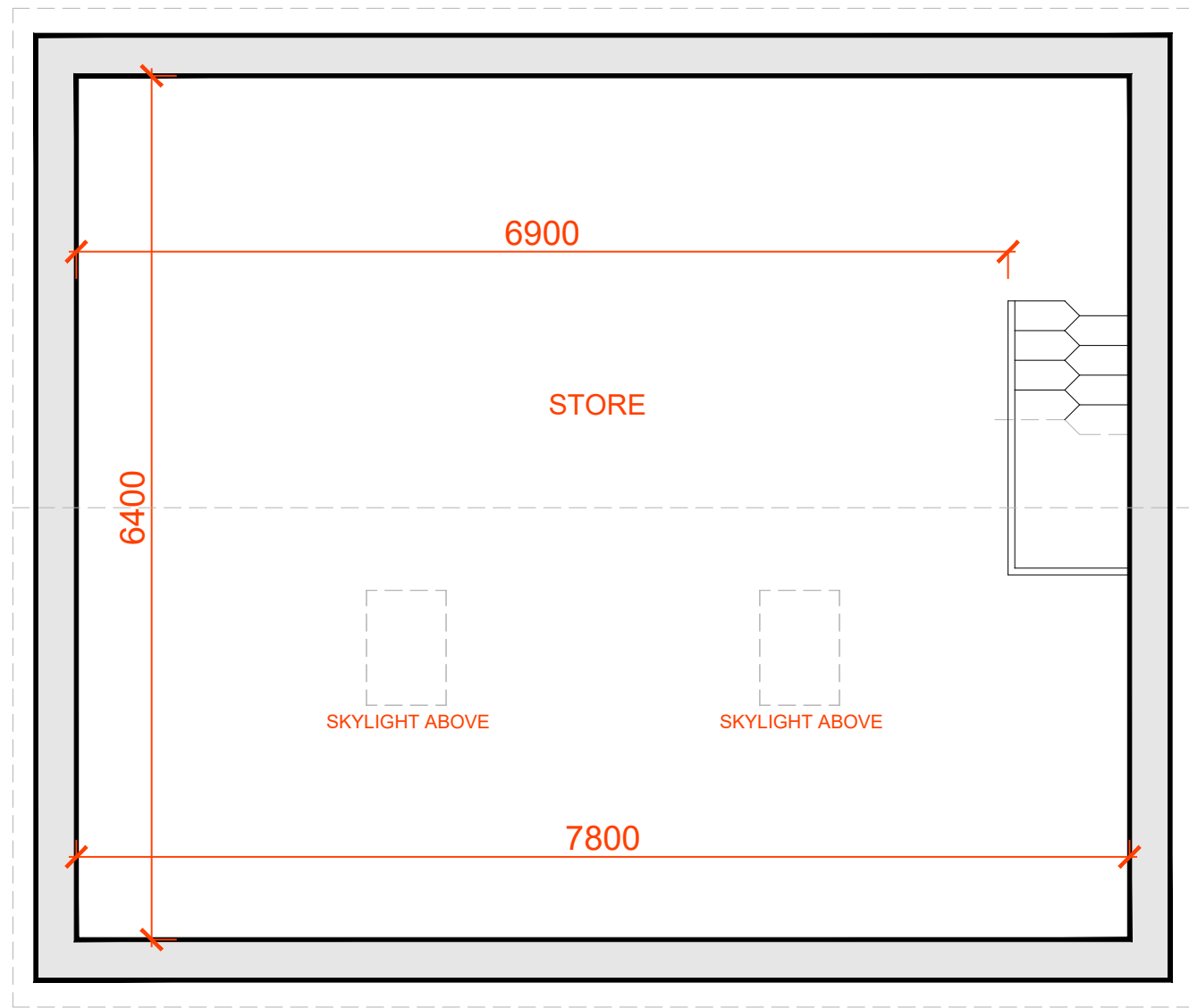
P2 Proposed First Plan (GIA 48sqm) 1:50@A1
