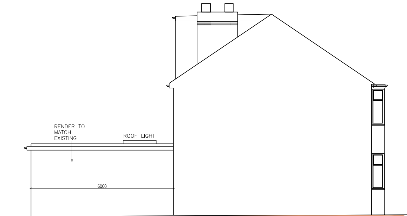
PROPOSED OTHER SIDE ELEVATION
