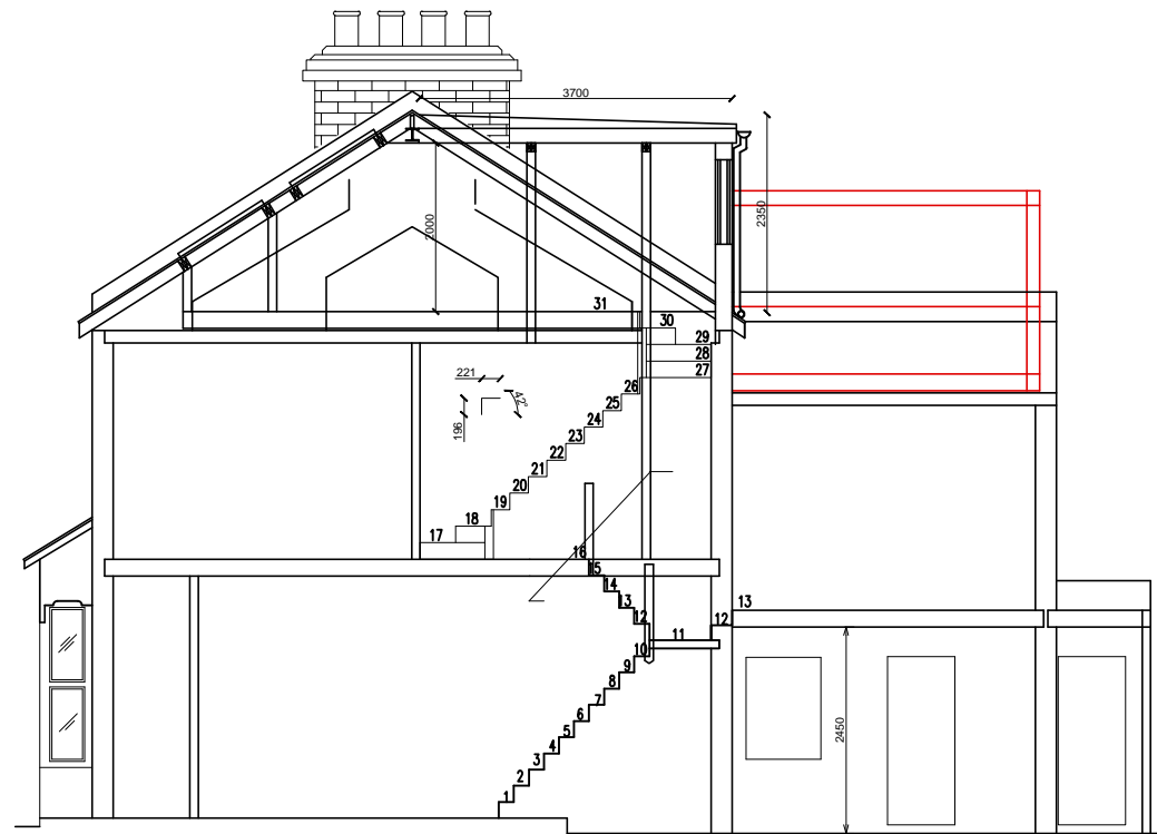
PROPOSED SECTION
