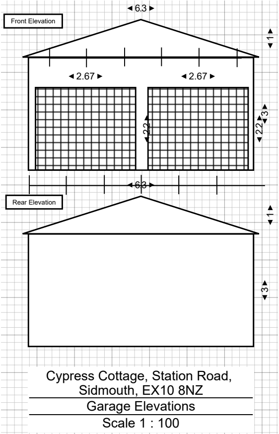
Proposed Elevations
