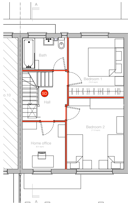
FIRST FLOOR PLAN Scale 1:100 @ A3
