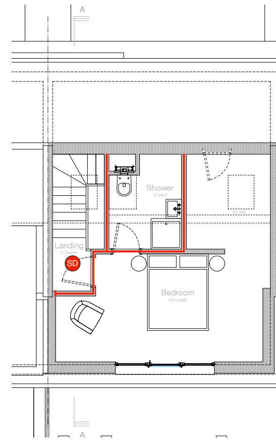
SECOND FLOOR PLAN Scale 1:100 @ A3
