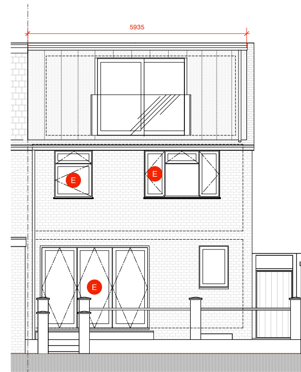
REAR ELEVATION Scale 1:100 @ A3
