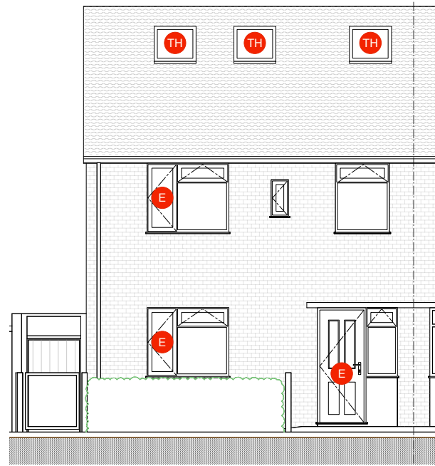
FRONT ELEVATION Scale 1:100 @ A3
