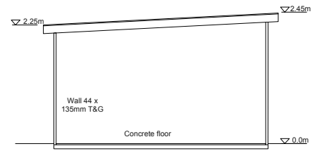
Proposed Section
