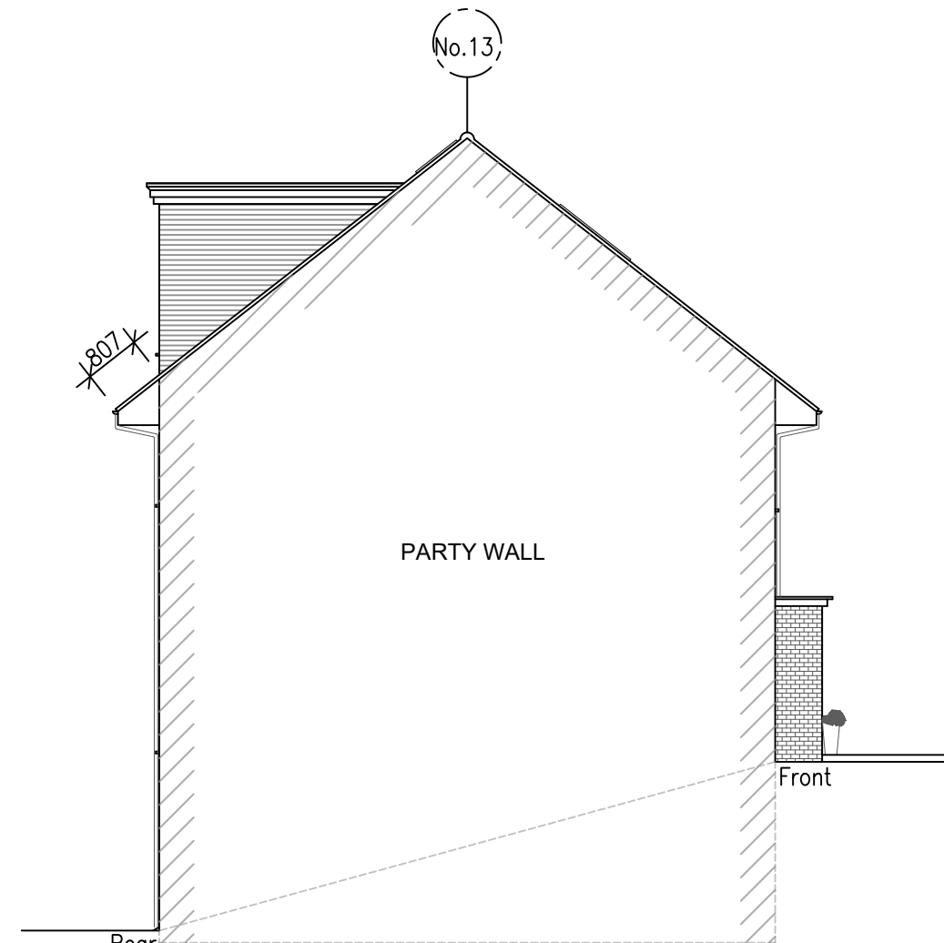
PROPOSED LEFT SIDE ELEVATION
