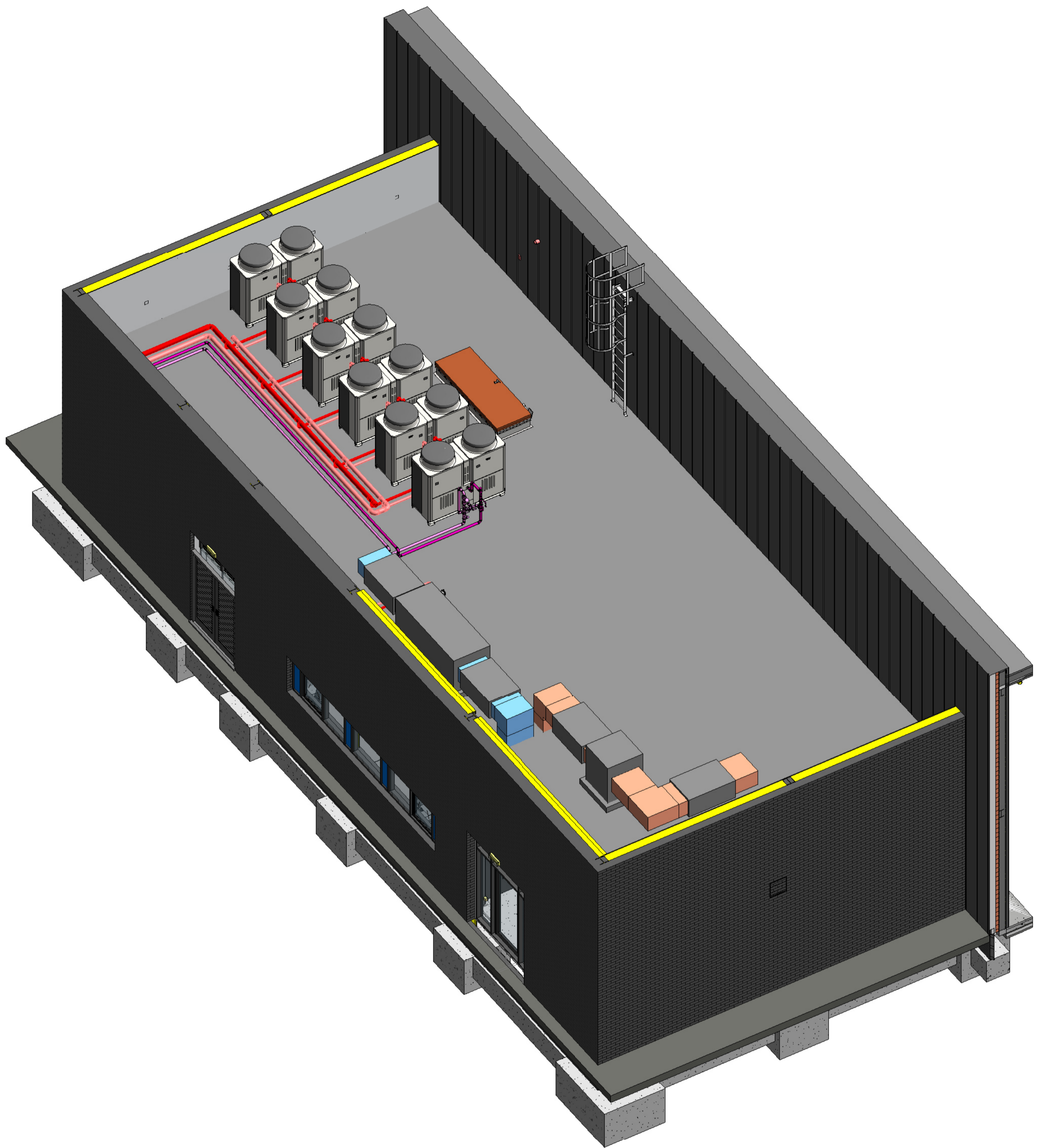
LEVEL 01 HEATING PLANTROOM 3D LAYOUT
