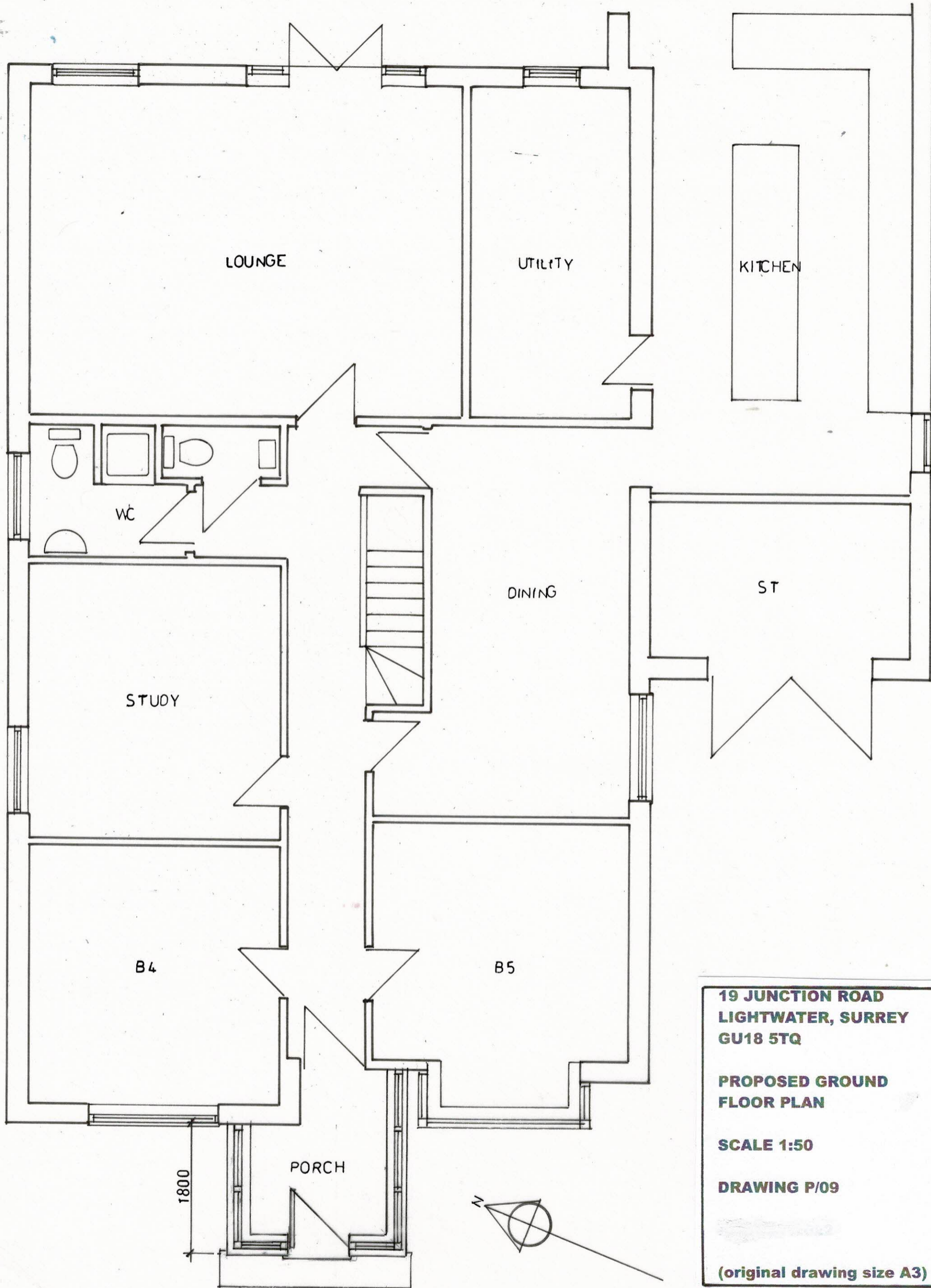
1 PROPOSED GROUND FLOOR PLAN 1: 50 0 1 2 3 4 5m
