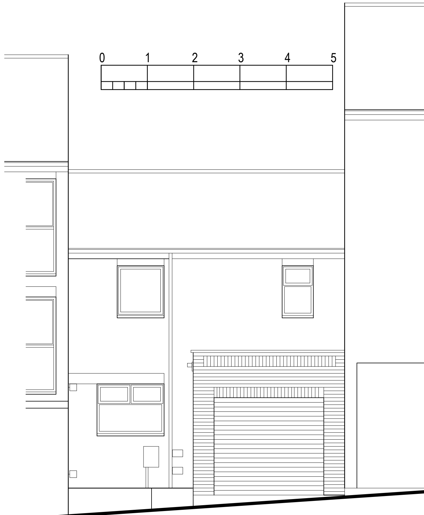
front elevation
