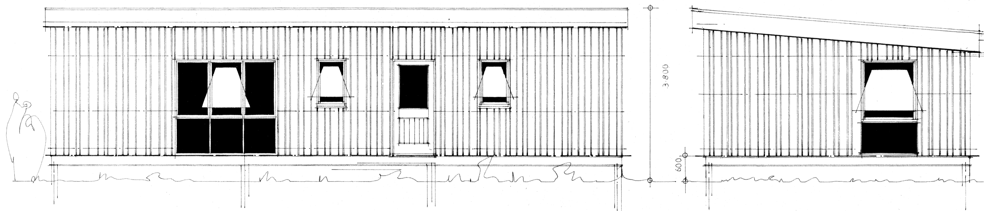
LODGE 1 WEST ELEVATION
