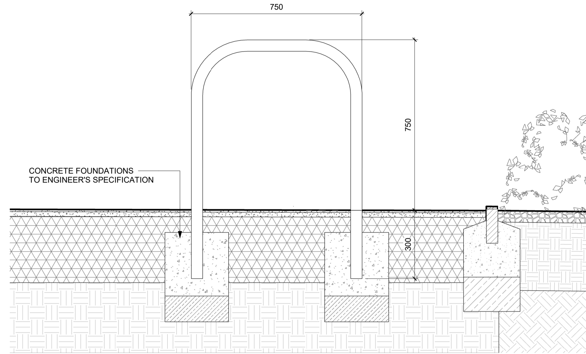
2 Typical Detail - Cycle hoop Scale 1 : 10
