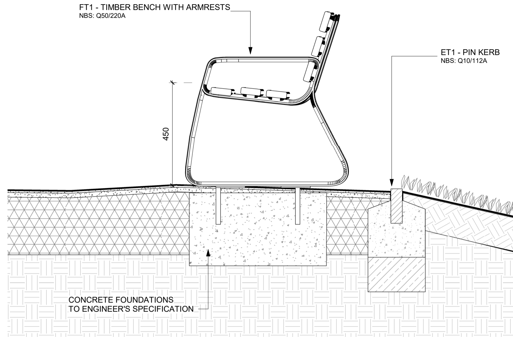
1 Typical Detail - Bench Scale 1 : 10
