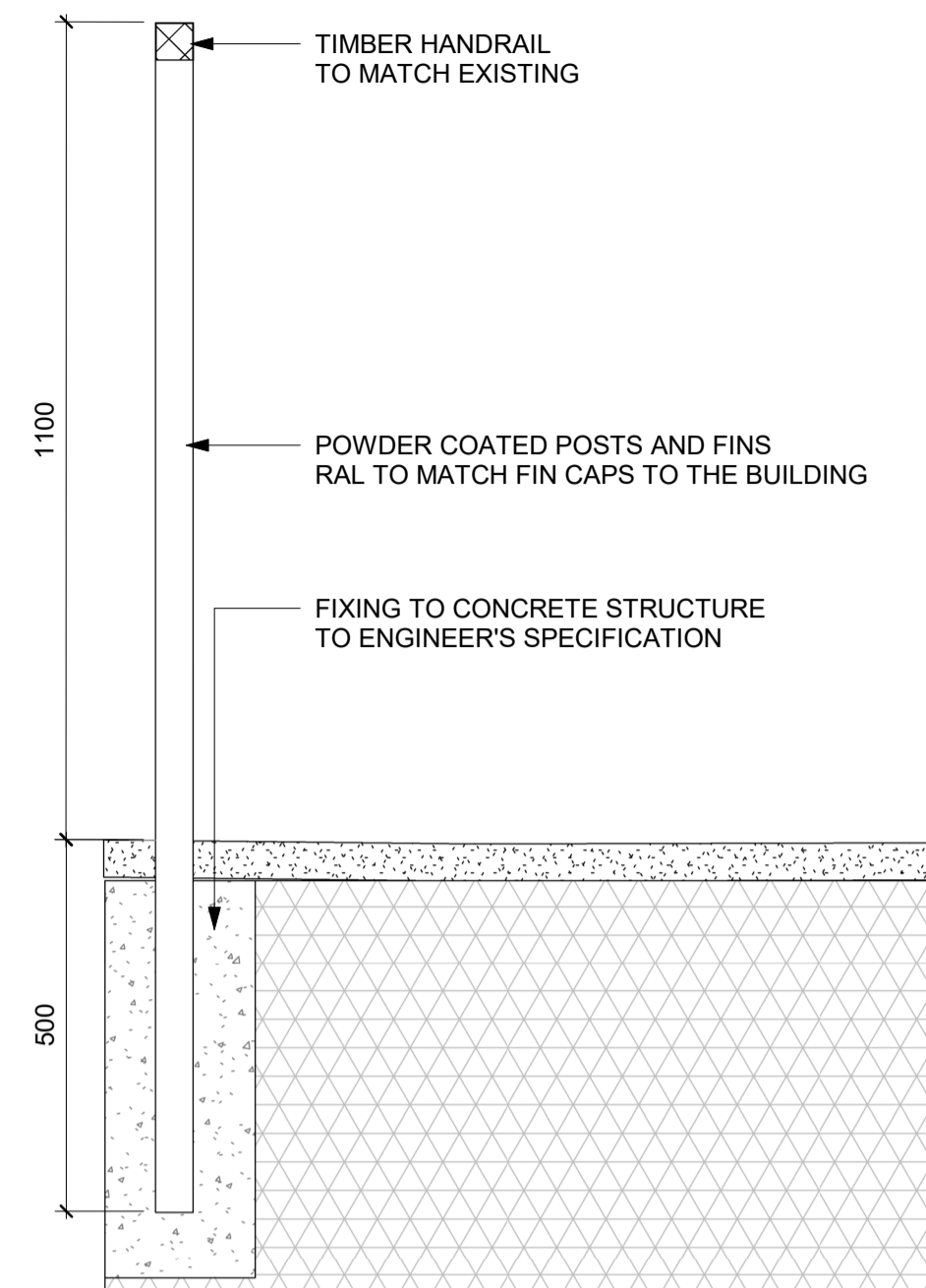
5 Typical Detail - BT1 Scale 1 : 10
