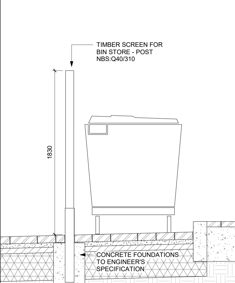
8 Typical Detail - BT2 fixing Scale 1 : 20
