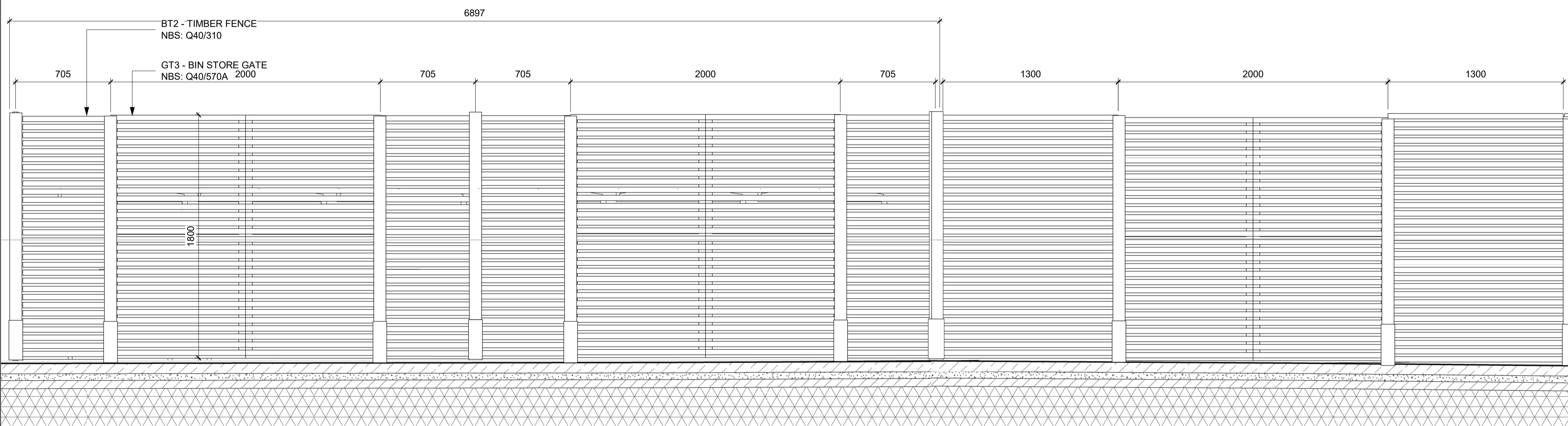
7 Bin Store - Elevation Scale 1 : 20
