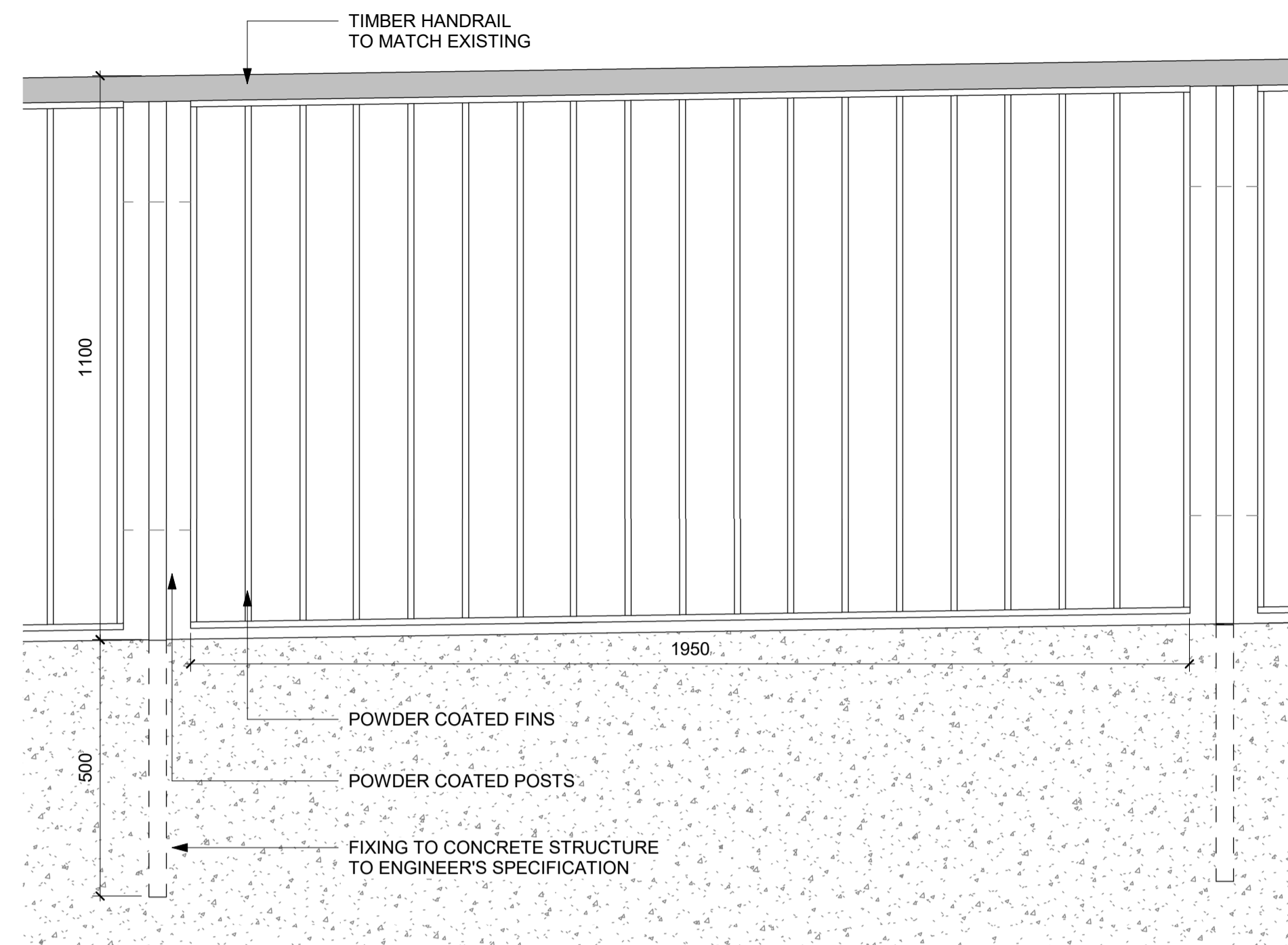
4 Typical Detail - BT1 Vertical Bar Railing Scale 1 : 10
