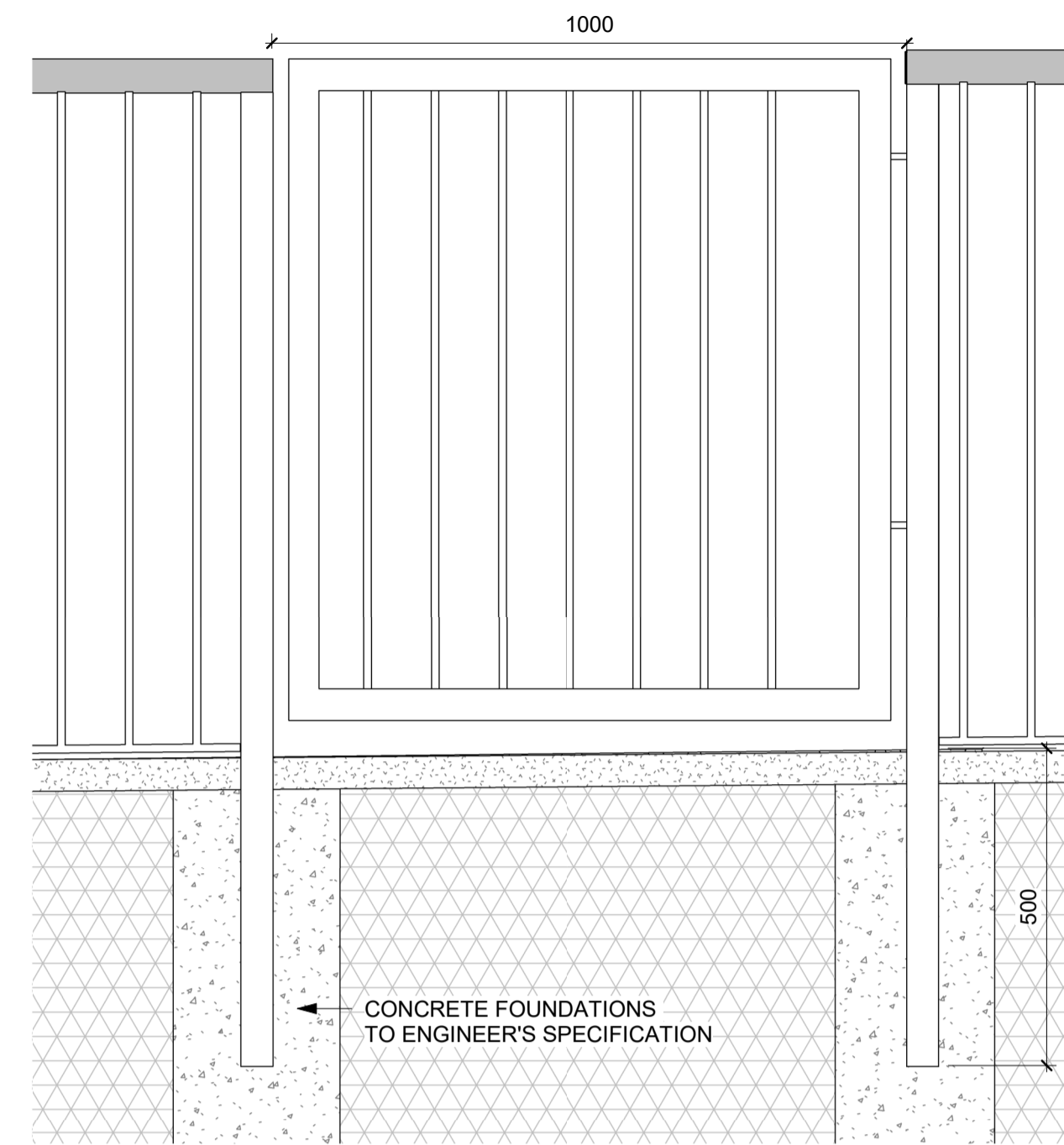
6 Typical Detail - GT2 Scale 1 : 10
