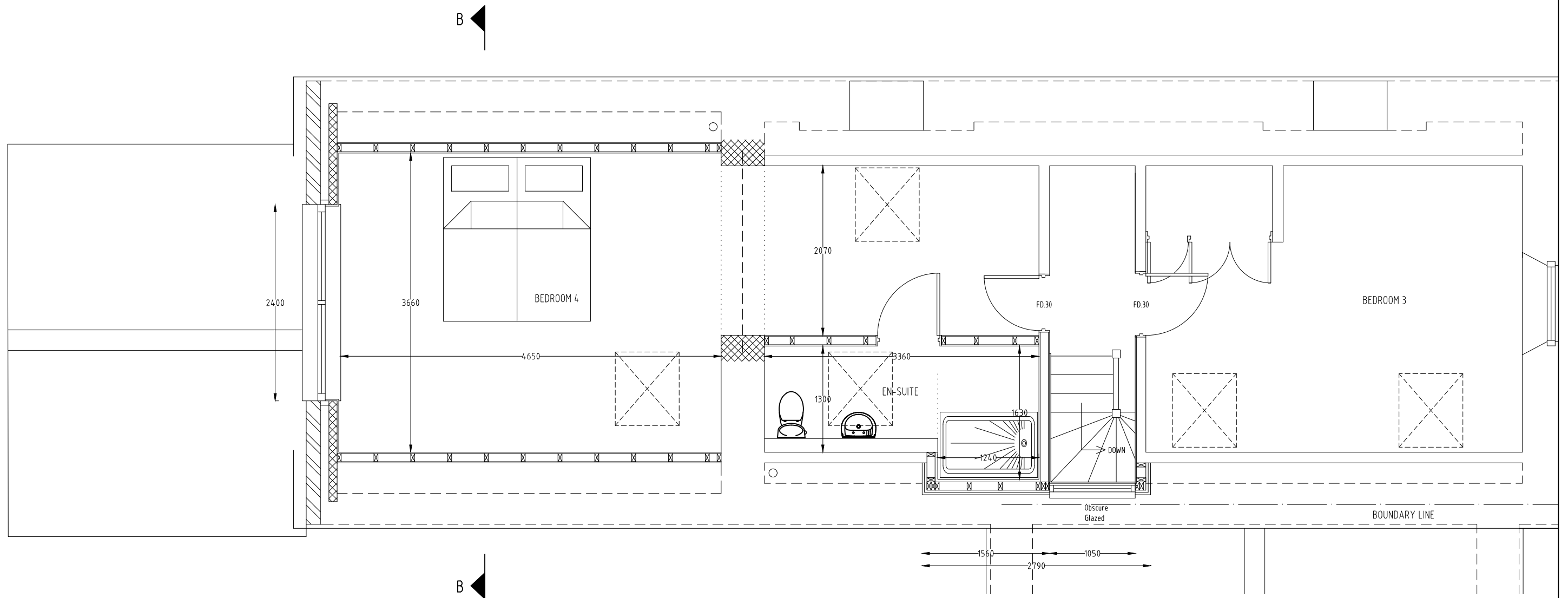
PROPOSED SECOND FLOOR PLAN SCALE 1:50
