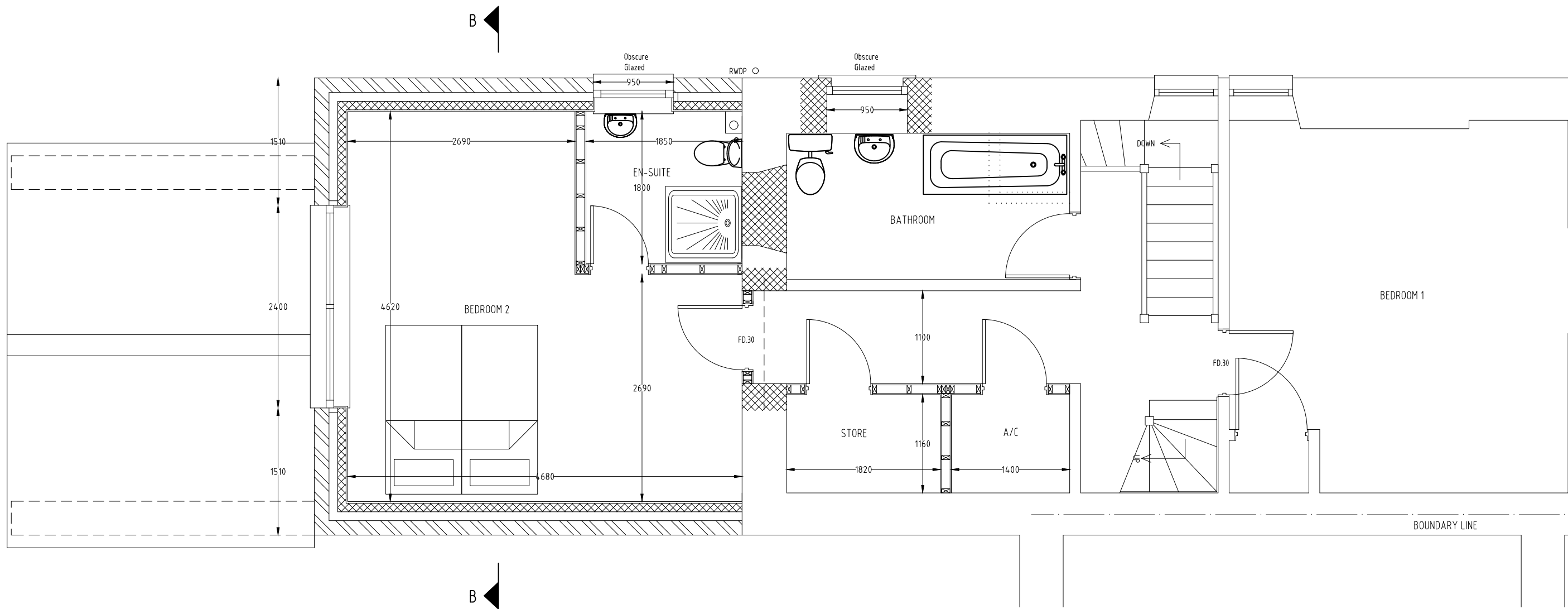
PROPOSED FIRST FLOOR PLAN SCALE 1:50
