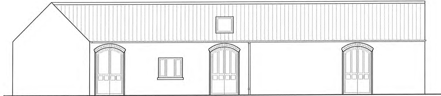
01 | EXISTING SOUTH ELEVATION Scale 1:50 @ A3
