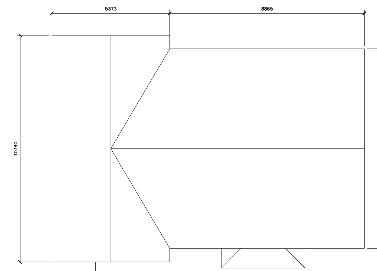
Roof plan
