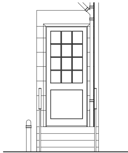
FRONT ELEVATION 1:50
