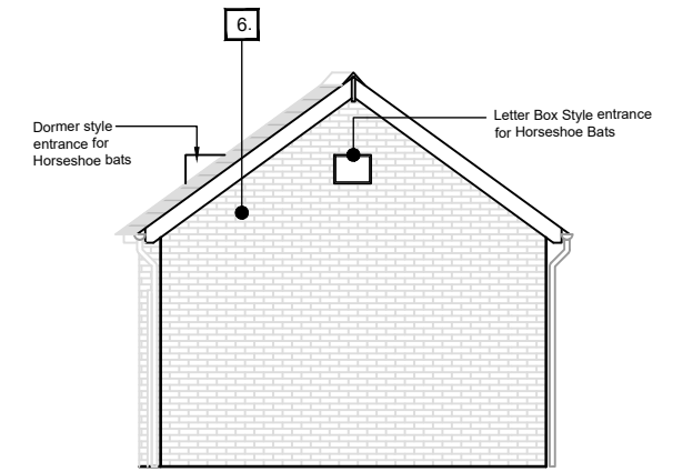
NEW BAT ROOST - NORTH ELEVATION
