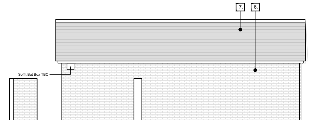
NEW BAT ROOST - WEST ELEVATION
