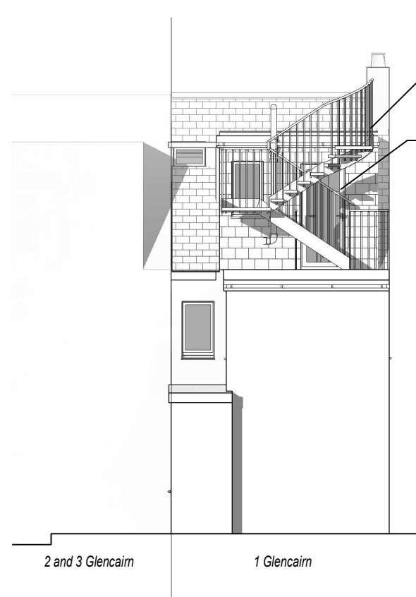
3 East Elevation 1 : 100
