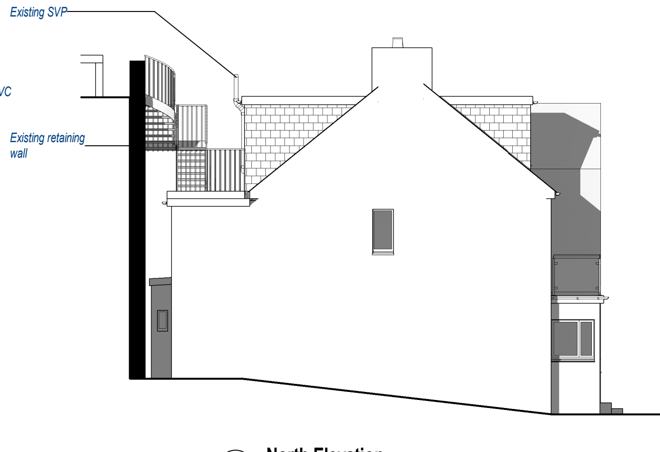
4 North Elevation 1 : 100
