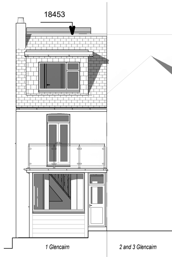
1 West Elevation 1 : 100
