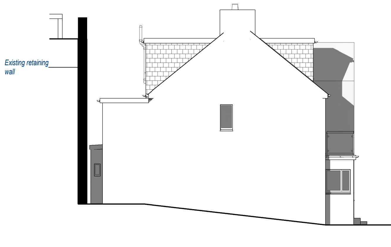
4 North Elevation 1 : 100
