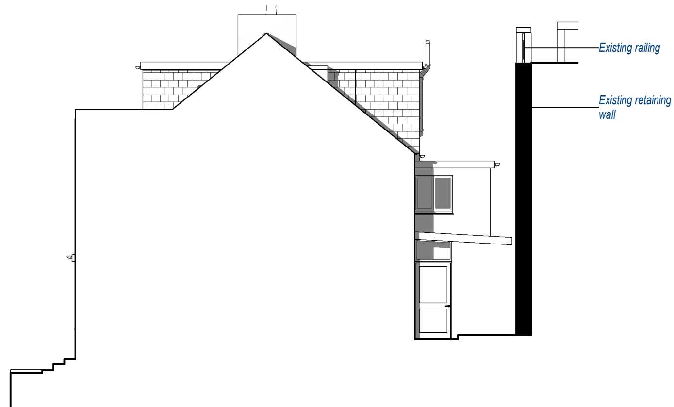
2 South Elevation 1 : 100
