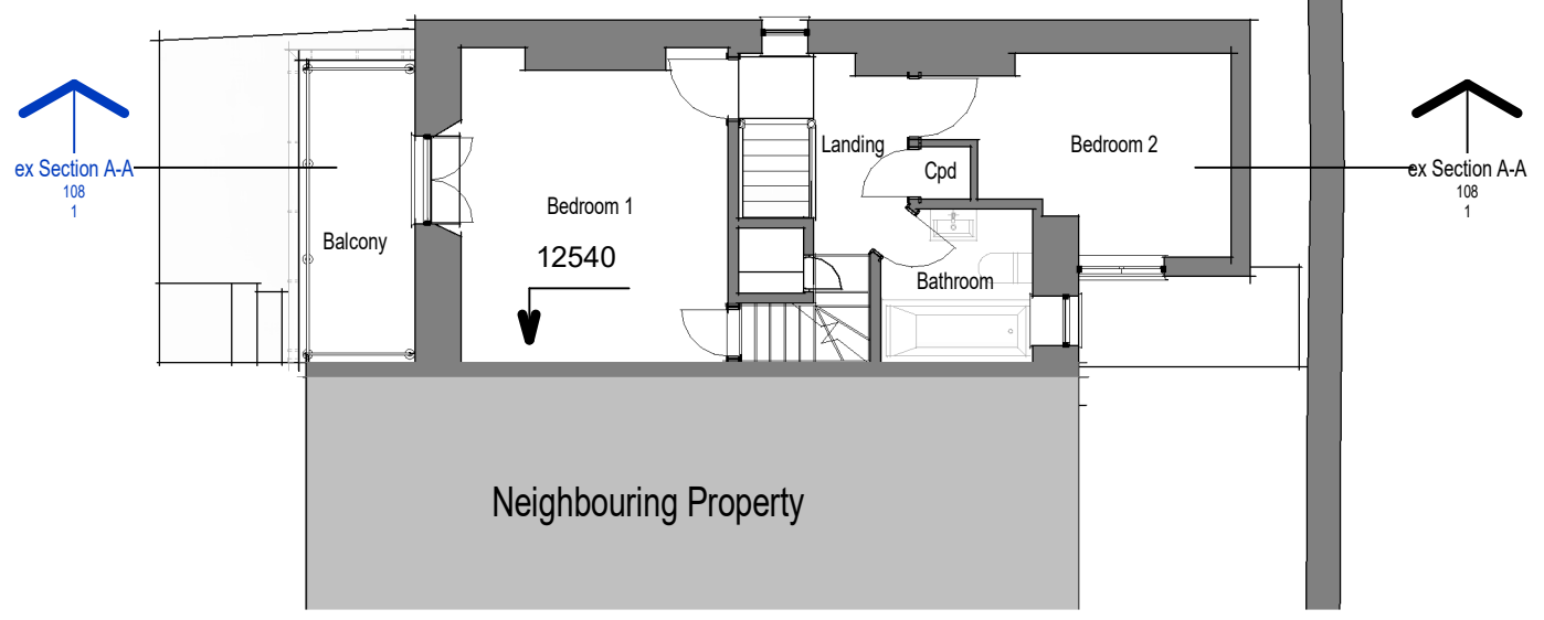
2 First Floor 1 : 100
