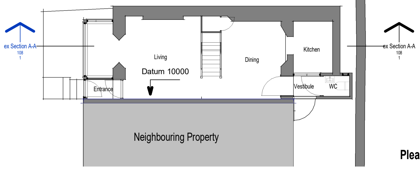
1 Ground Floor 1 : 100
