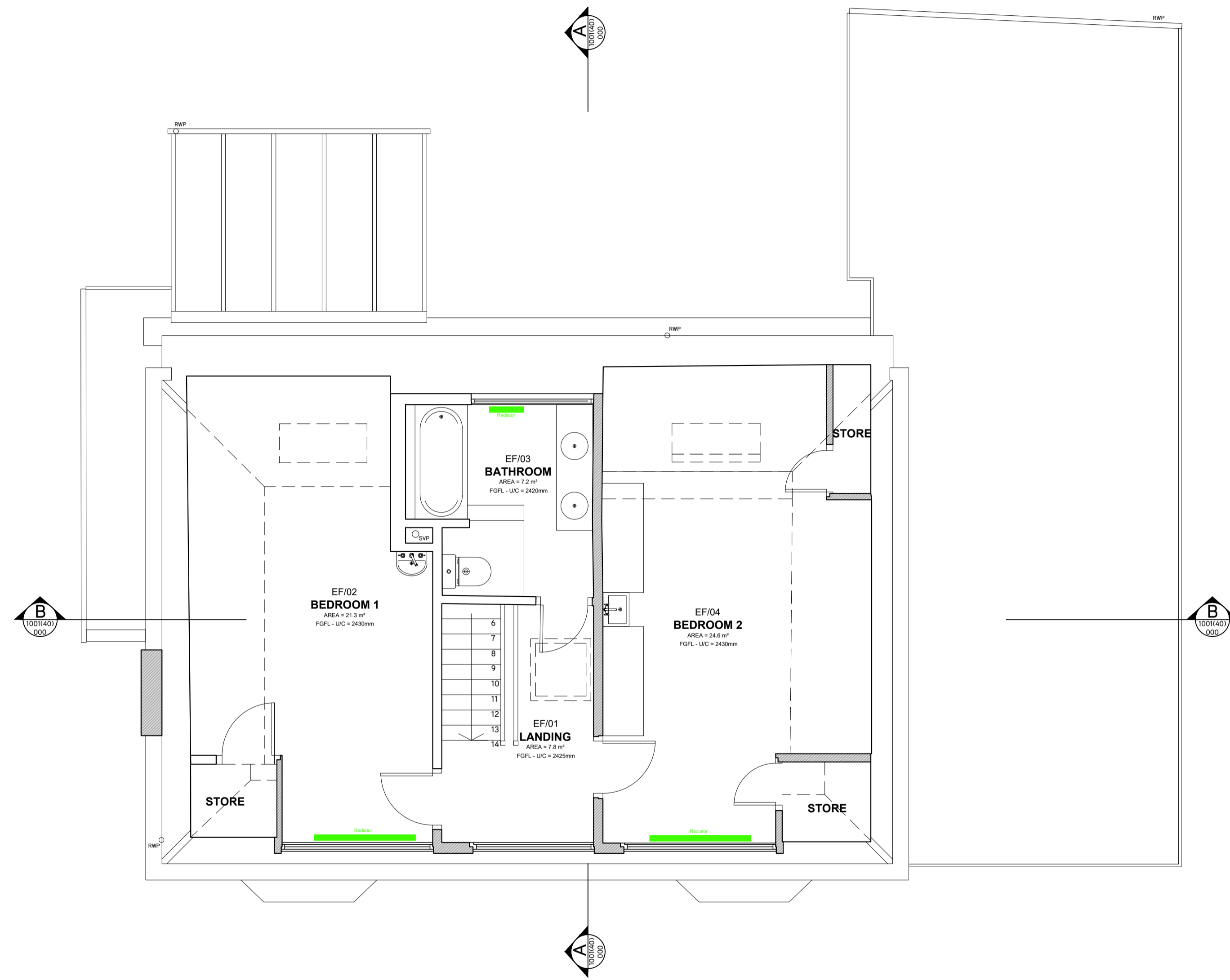
2 Existing First Floor Plan Scale 1:50 at A1 0 0.5 1.0 2.0 3.0 4.0 5.0 Scale in metres
