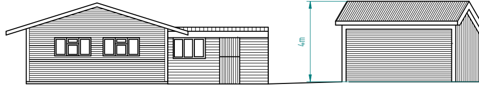
WEST ELEVATION
