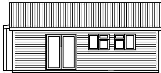
NORTH ELEVATION
