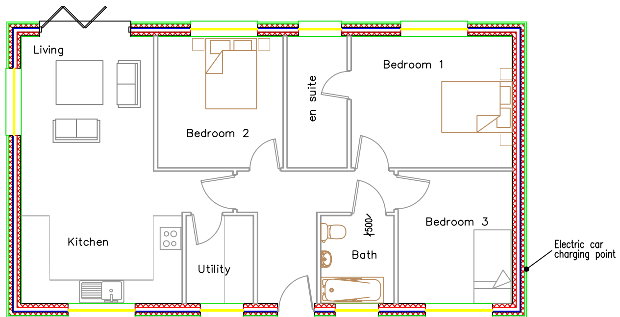
Floor Plan – GIA 96 sq m
