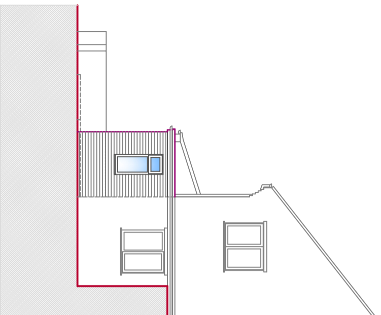
SITE CROSS-SECTION B-B / SIDE ELEVATION - As Proposed
