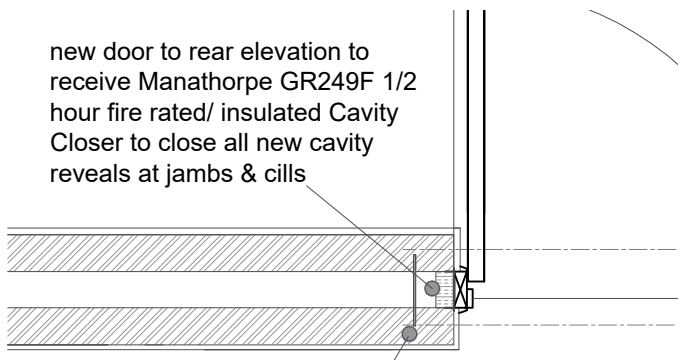
proposed door head detail
