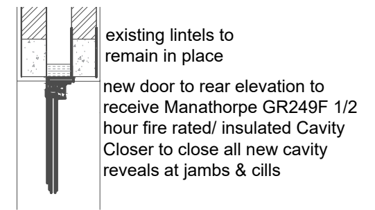
proposed door head detail
