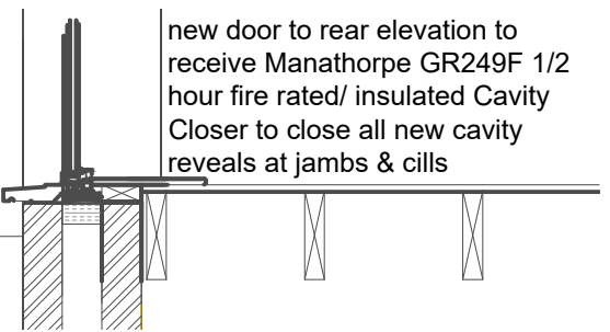
proposed door threshold detail
