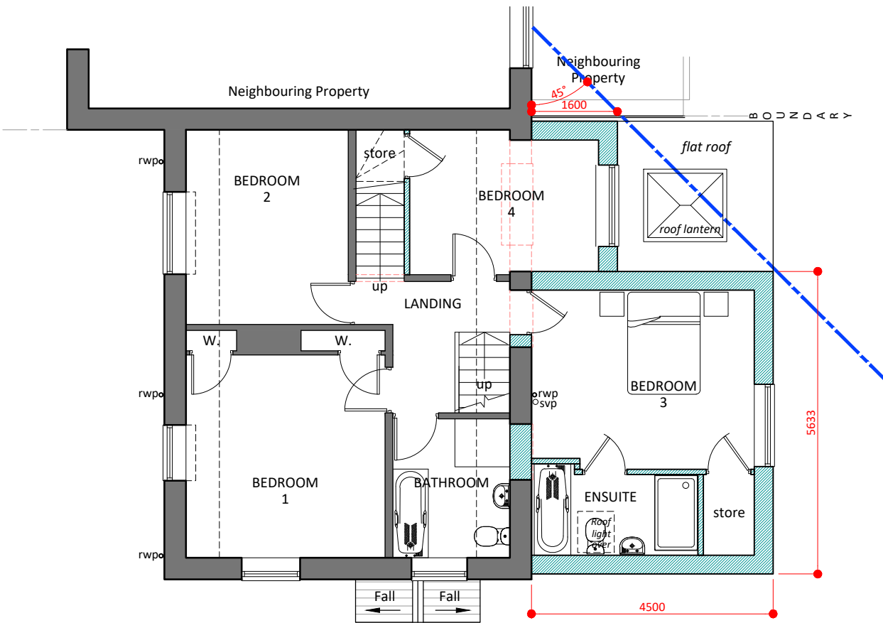
01 FIRST FLOOR PLAN 1:100
