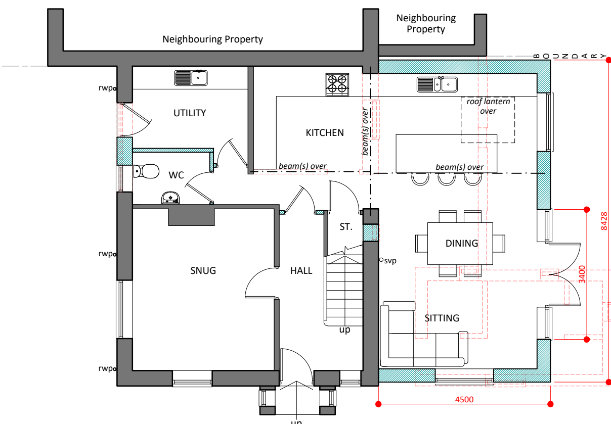
00 GROUND FLOOR PLAN 1:100
