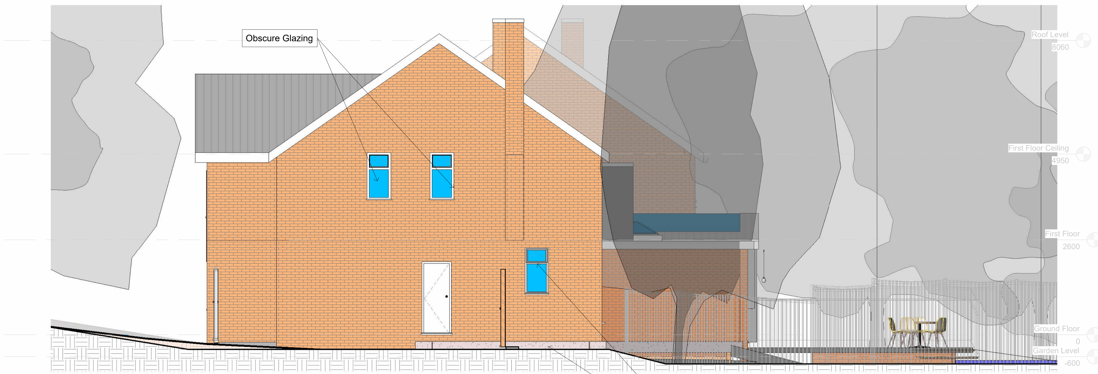
2 Proposed RHS Elevation 1 : 50
