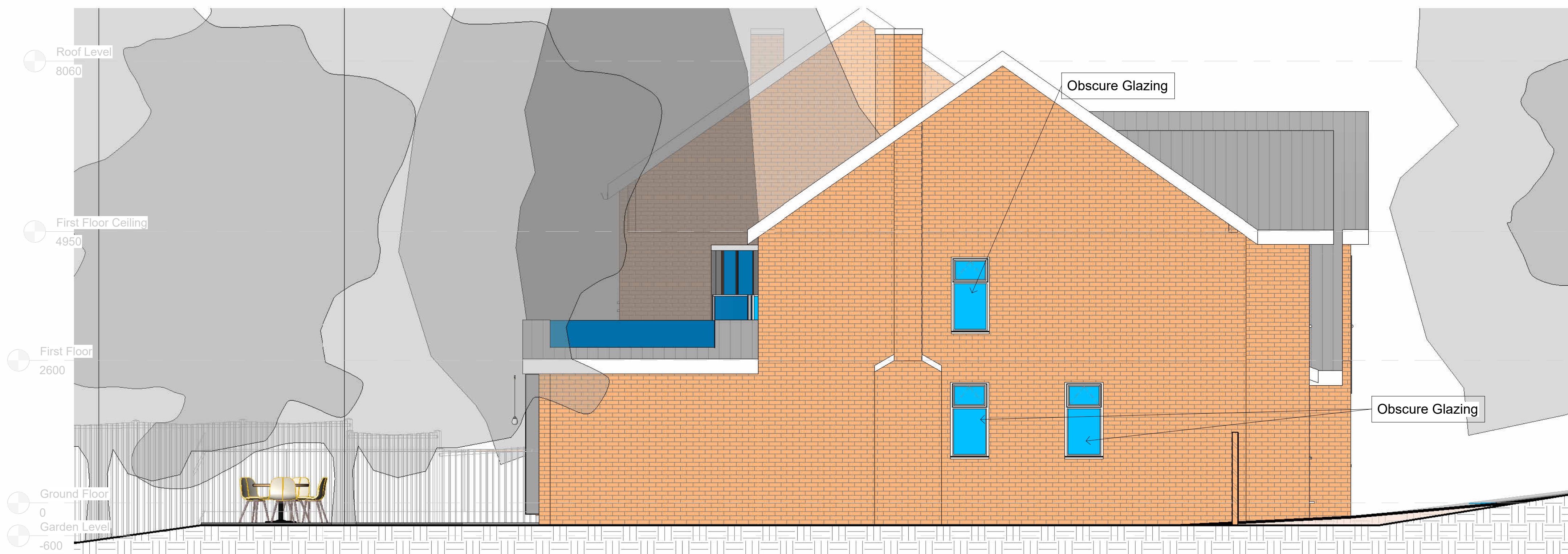
1 Proposed LHS Elevation 1 : 50
