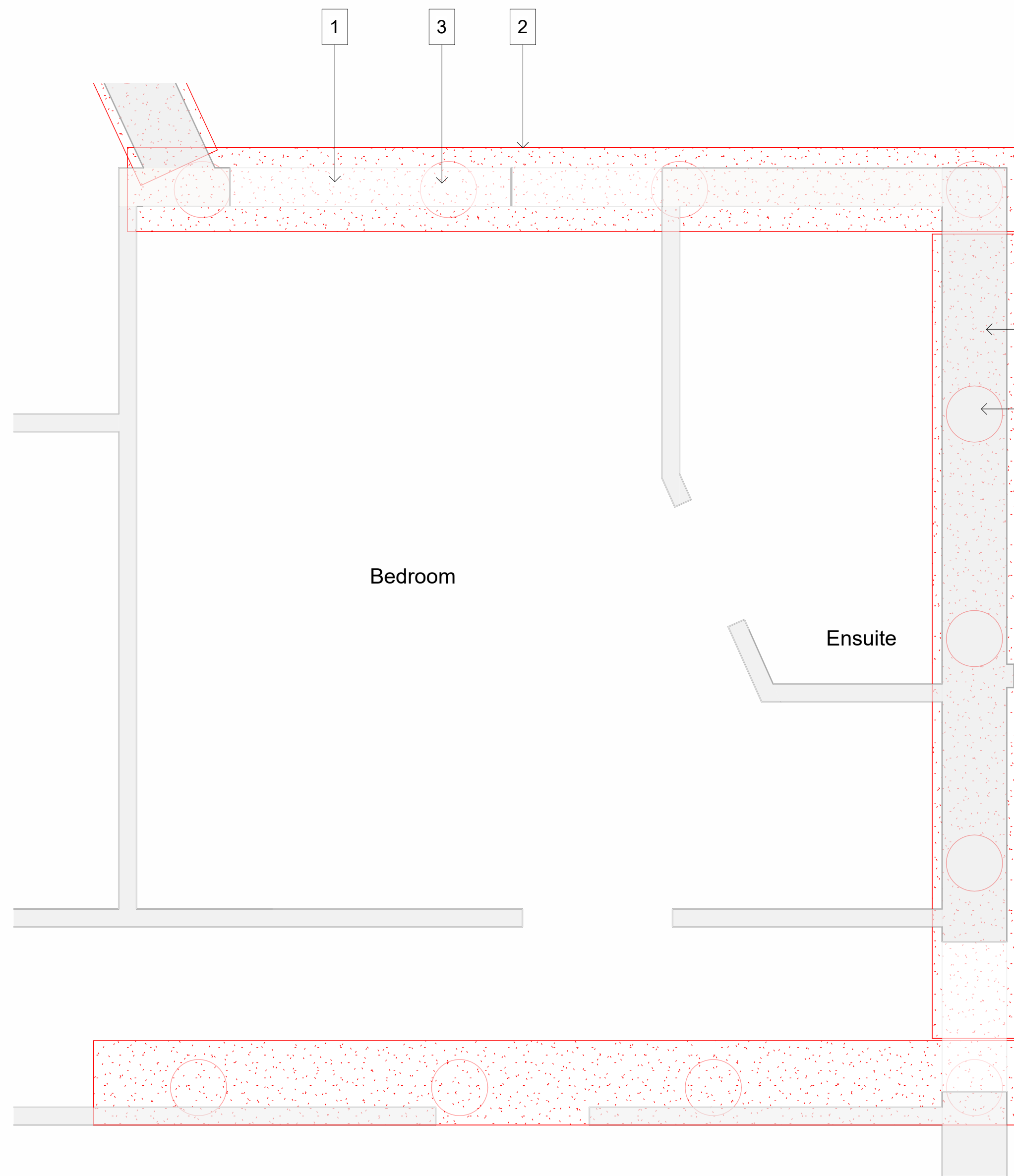
1 Proposed Ground Floor Structural Foundation - Pile Detail 1 : 20
