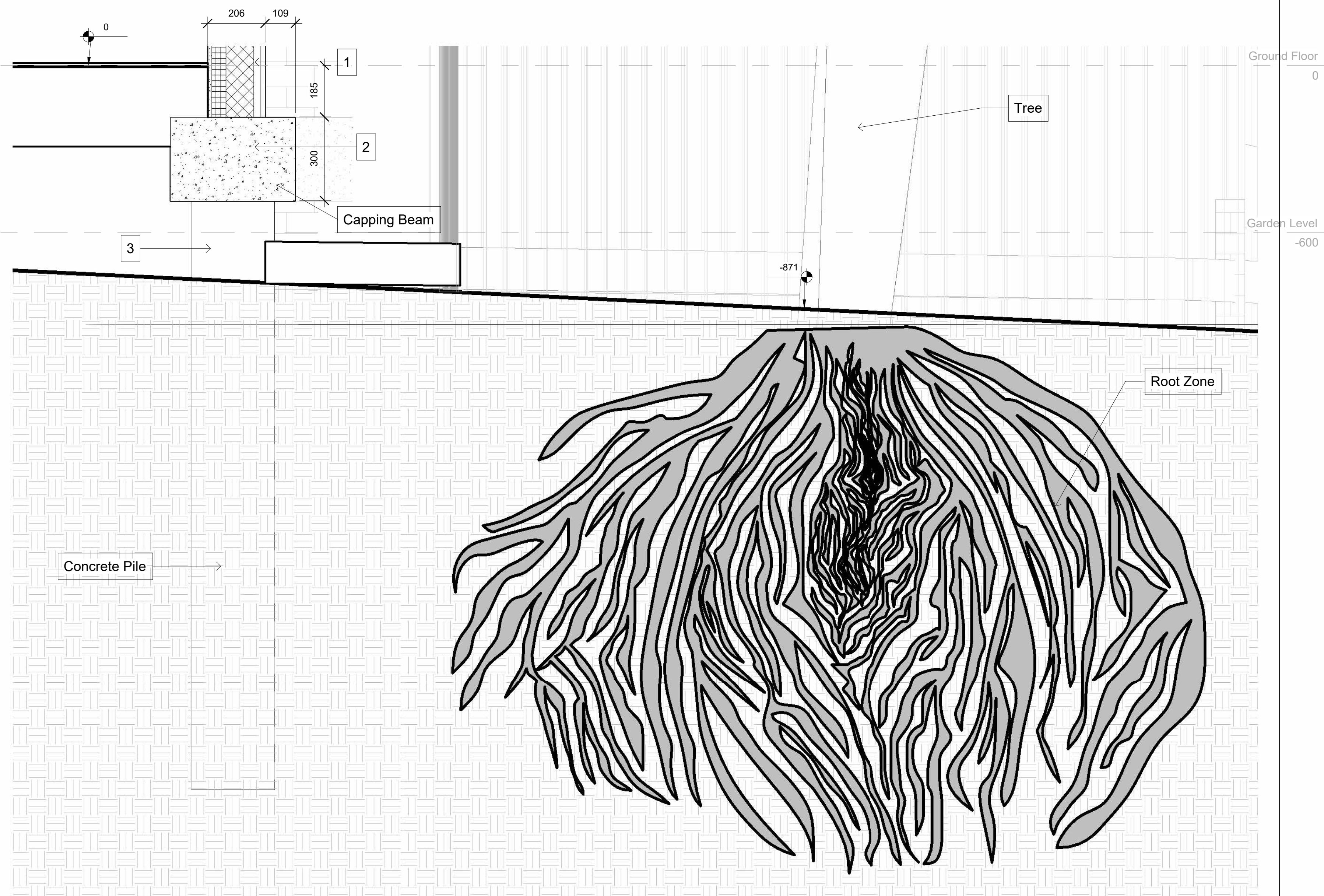
2 Proposed Section - Callout 1 1 : 10
