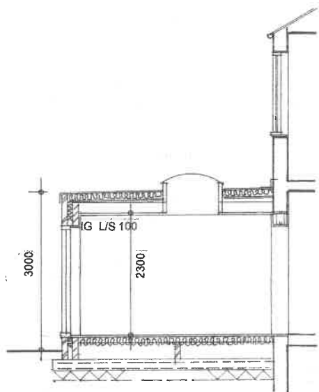
SECTION THRO EXTENSION
