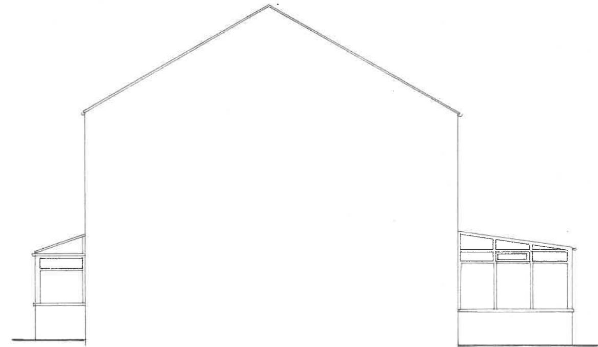
SOUTH ELEVATIONS
