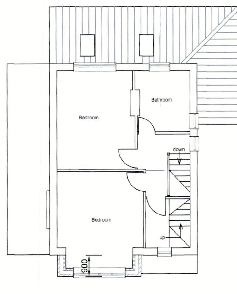
Proposed F.F. Plan View
