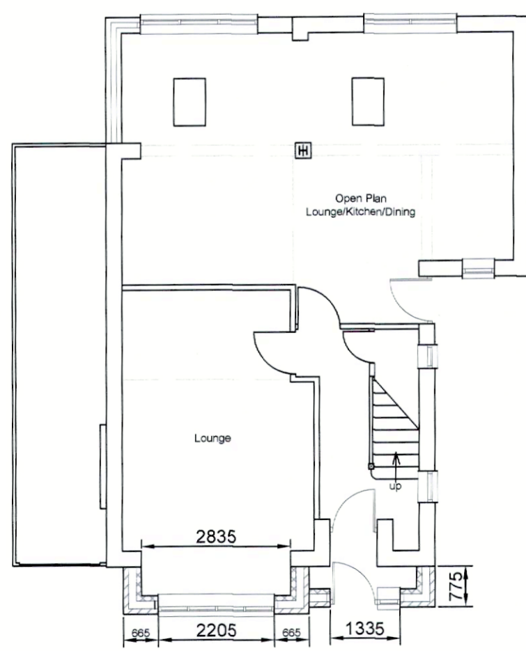
Proposed G.F. Plan View
