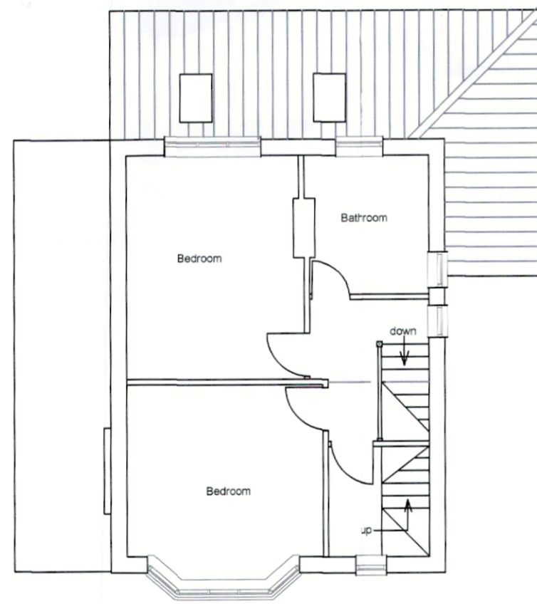
Existing F.F. Plan View
