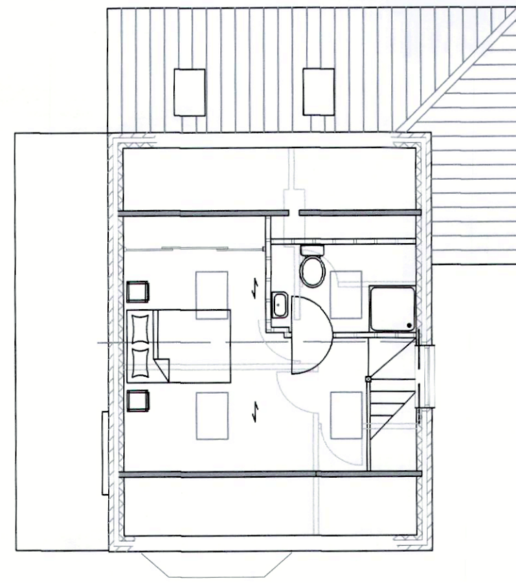
Existing 2nd Floor Plan View As 2020/0236 /HHA
