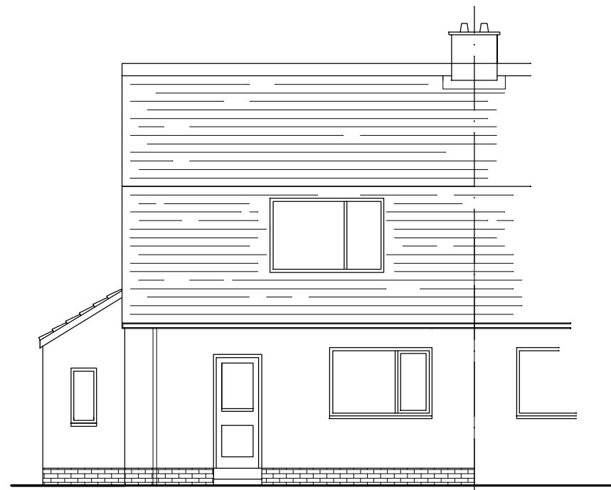
Front Elevation As Existing
