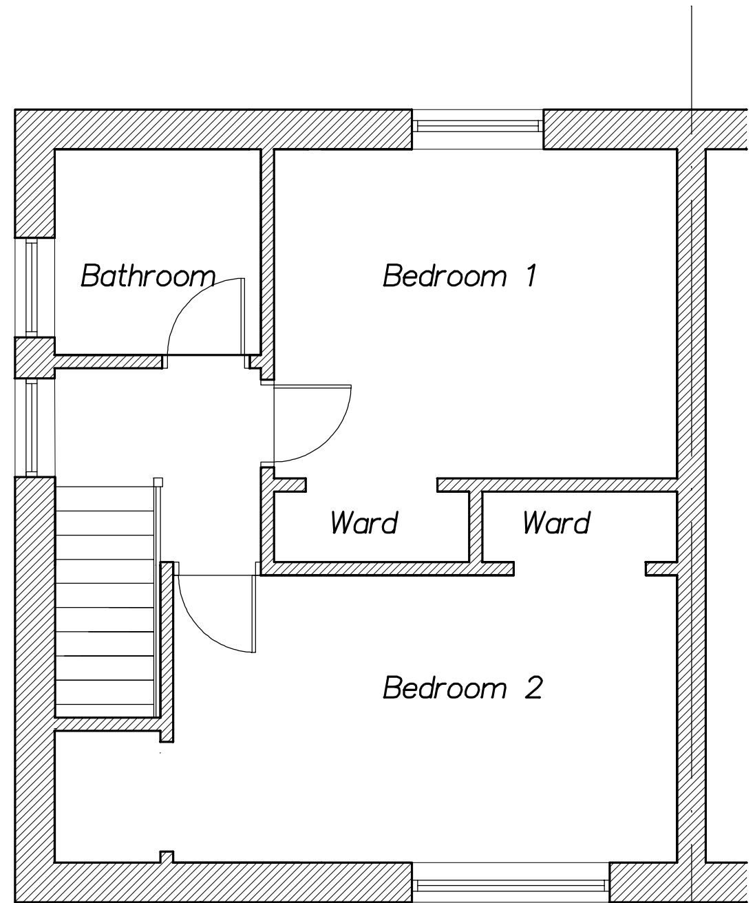
Upper Floor Plan As Existing
