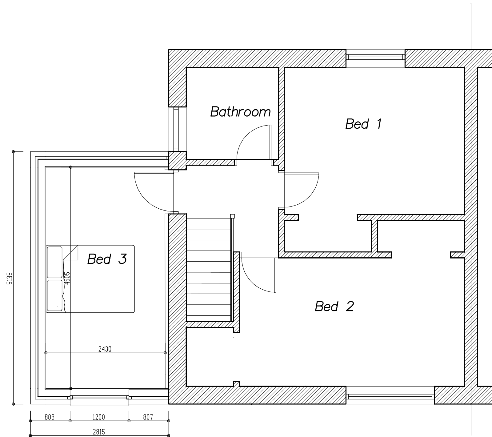
Upper Floor Plan As Proposed
