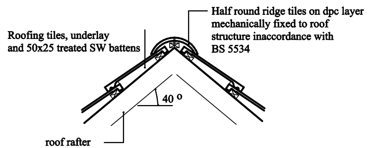
Section thro' ridge 40 degree tiled roof
