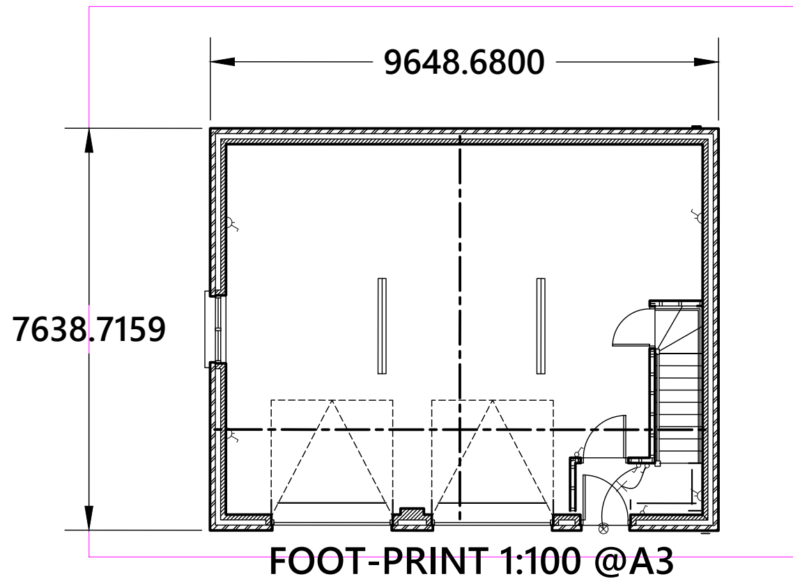
Proposed New Garage , 1200mm from Boundries
