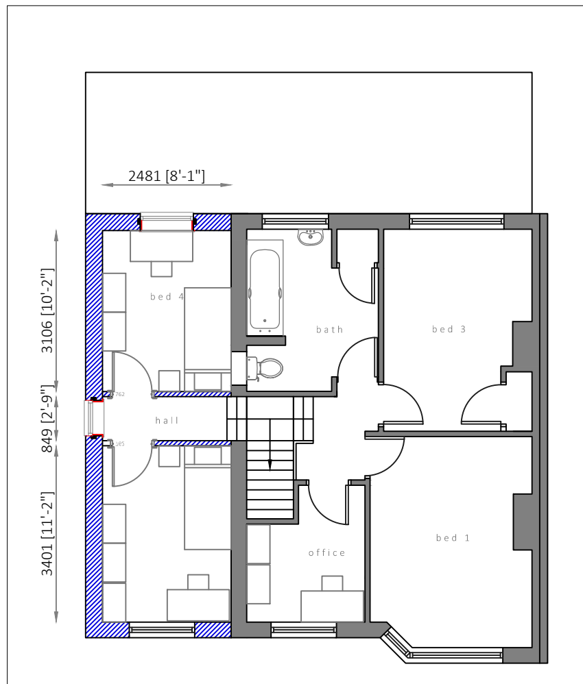
first floor
