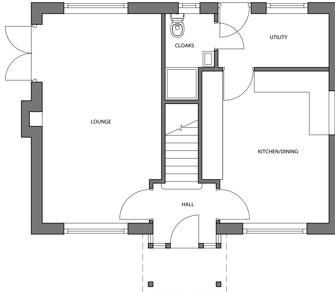
01 GROUND FLOOR PLAN -- 1:50
