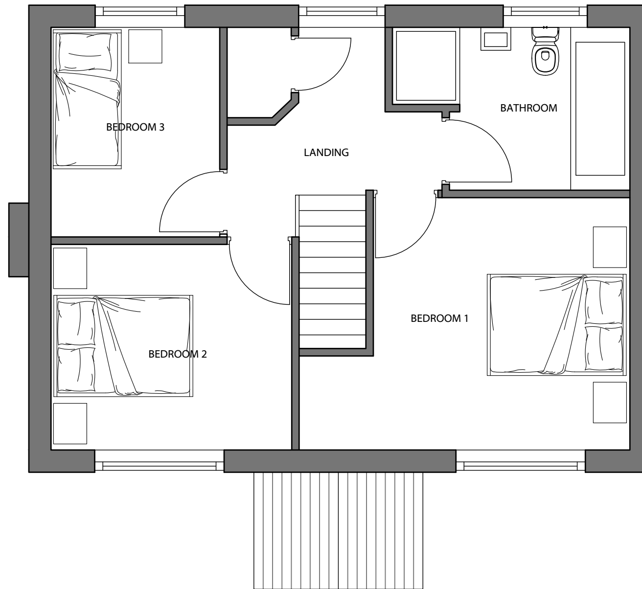
01 FIRST FLOOR PLAN -- 1:50
