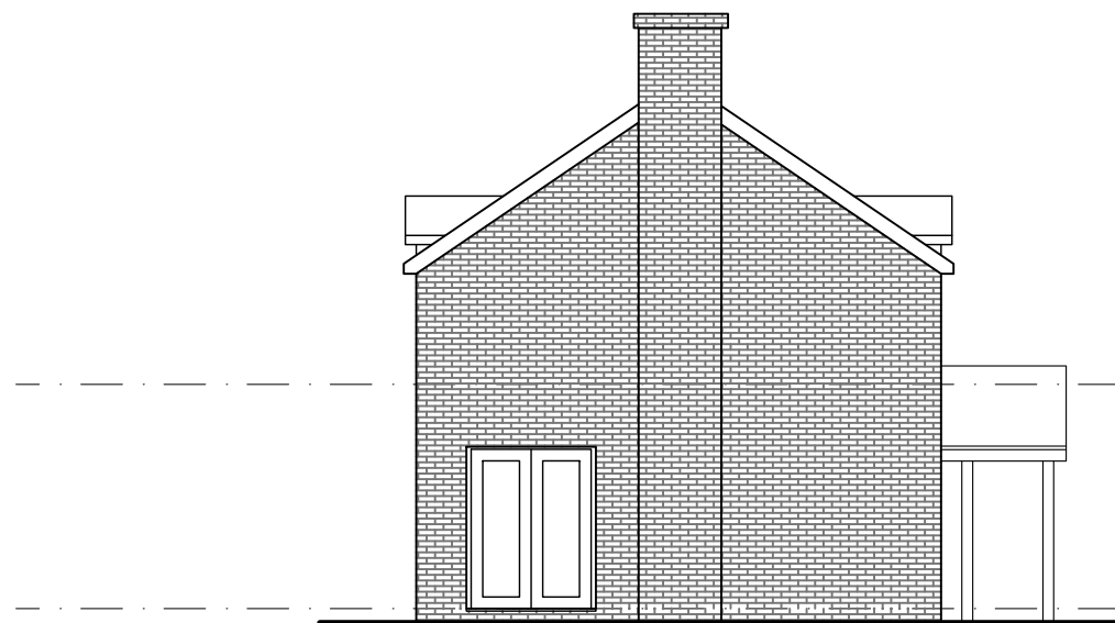
03 WEST ELEVATION 1:100
