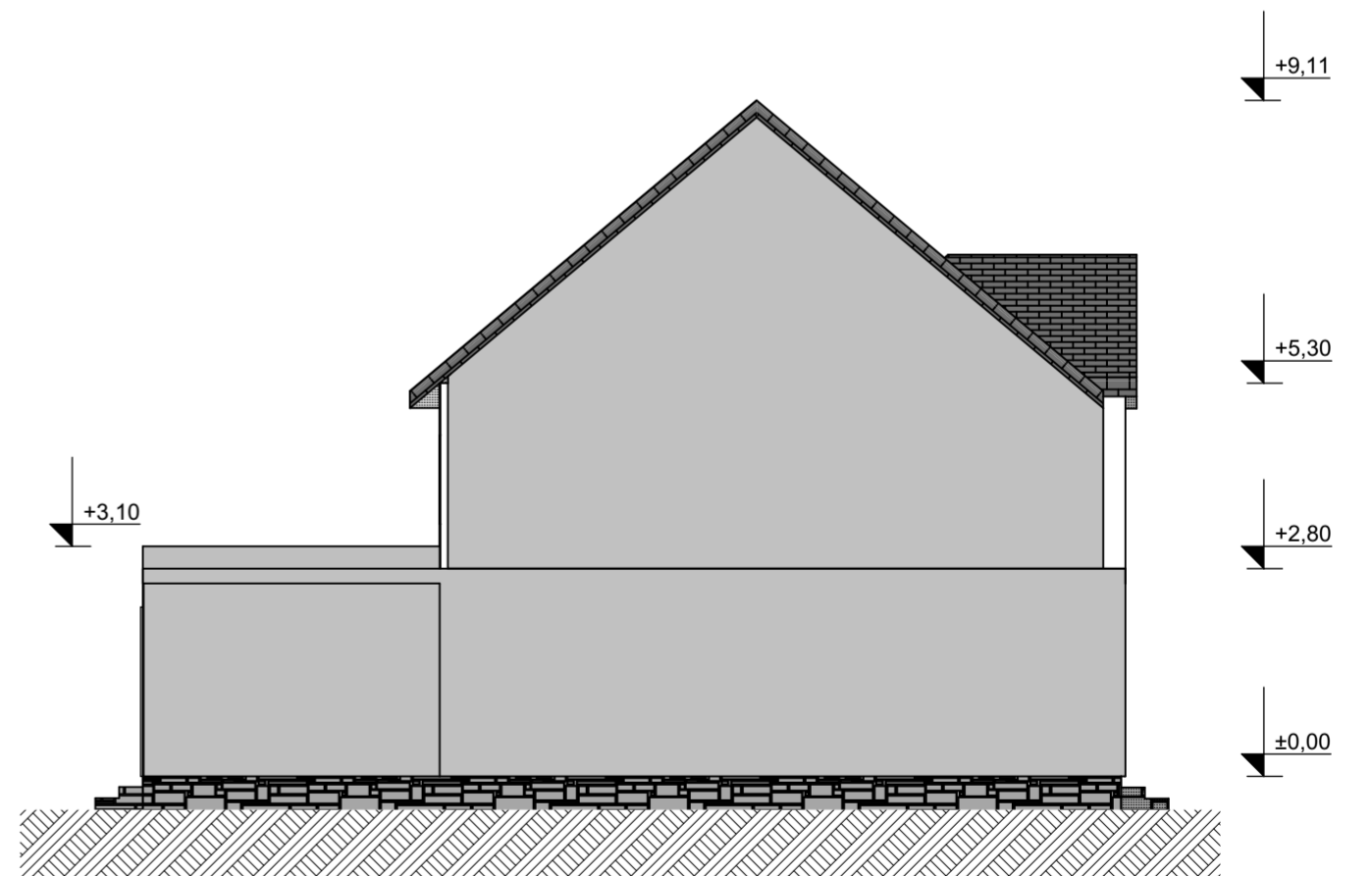
WEST ELEVATION RENOVATION M 1:100
