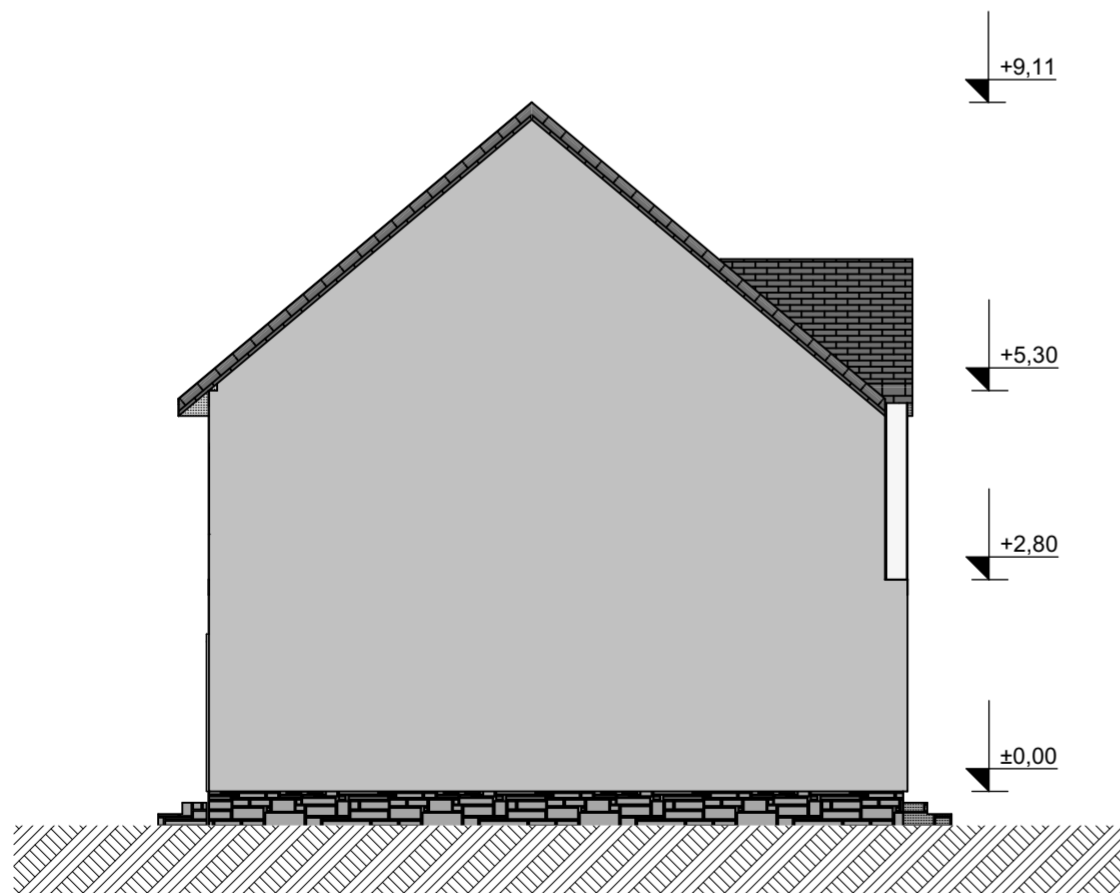
WEST ELEVATION M 1:100
