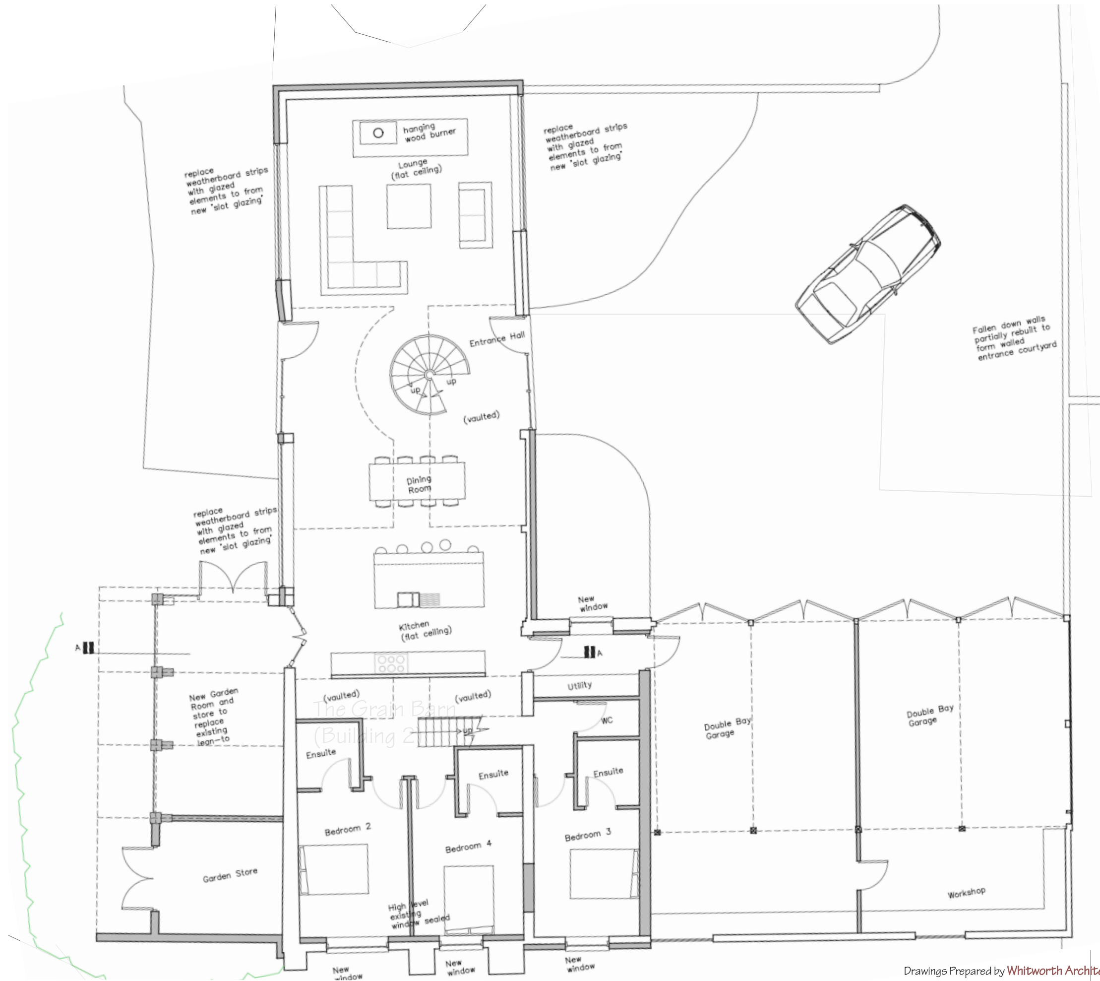
The Grain Barn Ground Floor Plan
