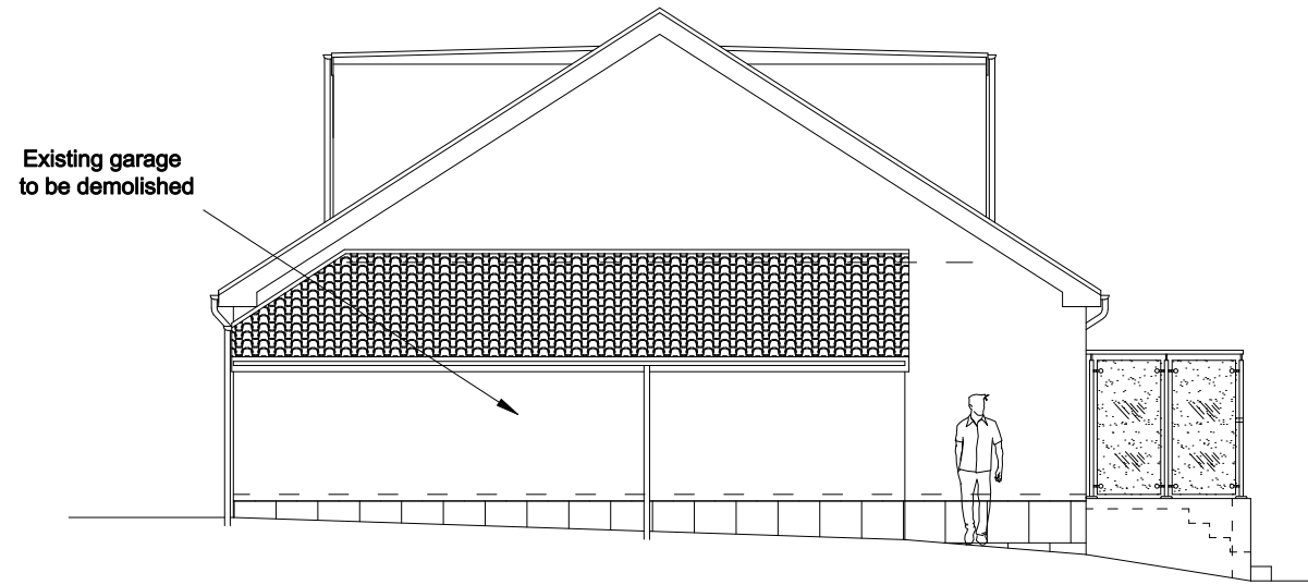
View A - Existing
