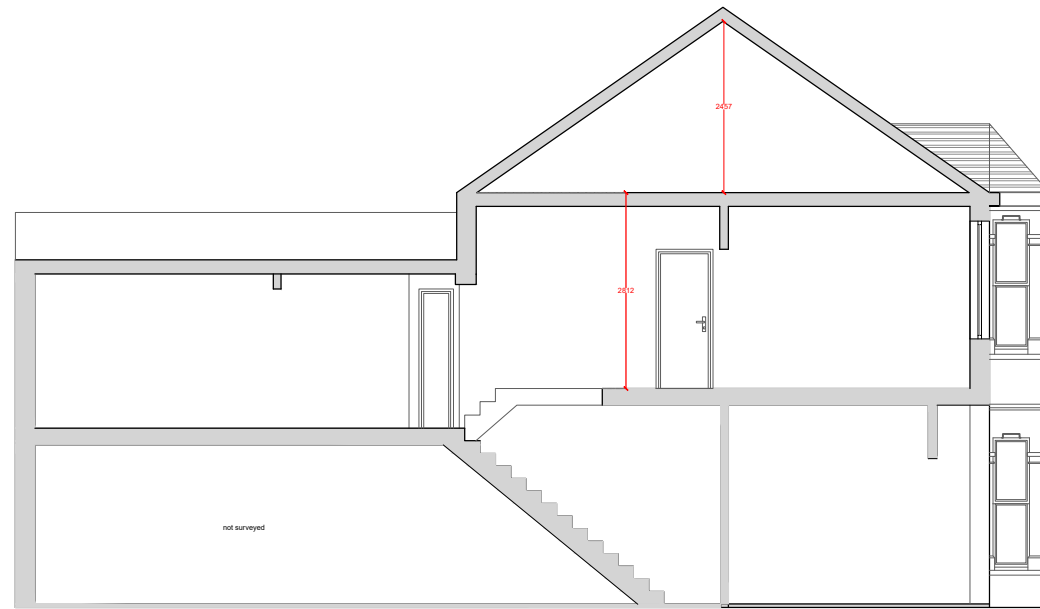
(AA) EXISTING SECTION AA
