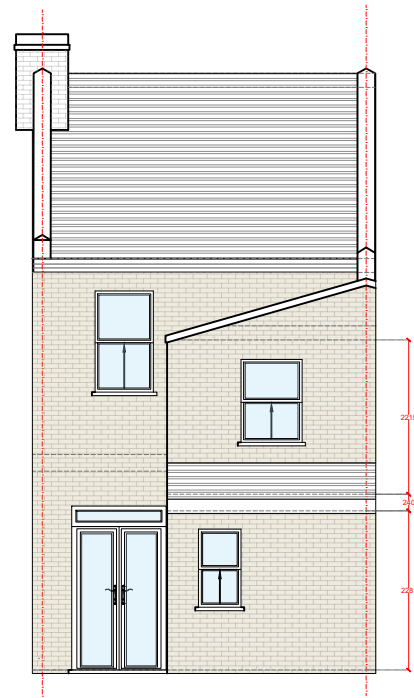
(B) EXISTING ELEVATION B
