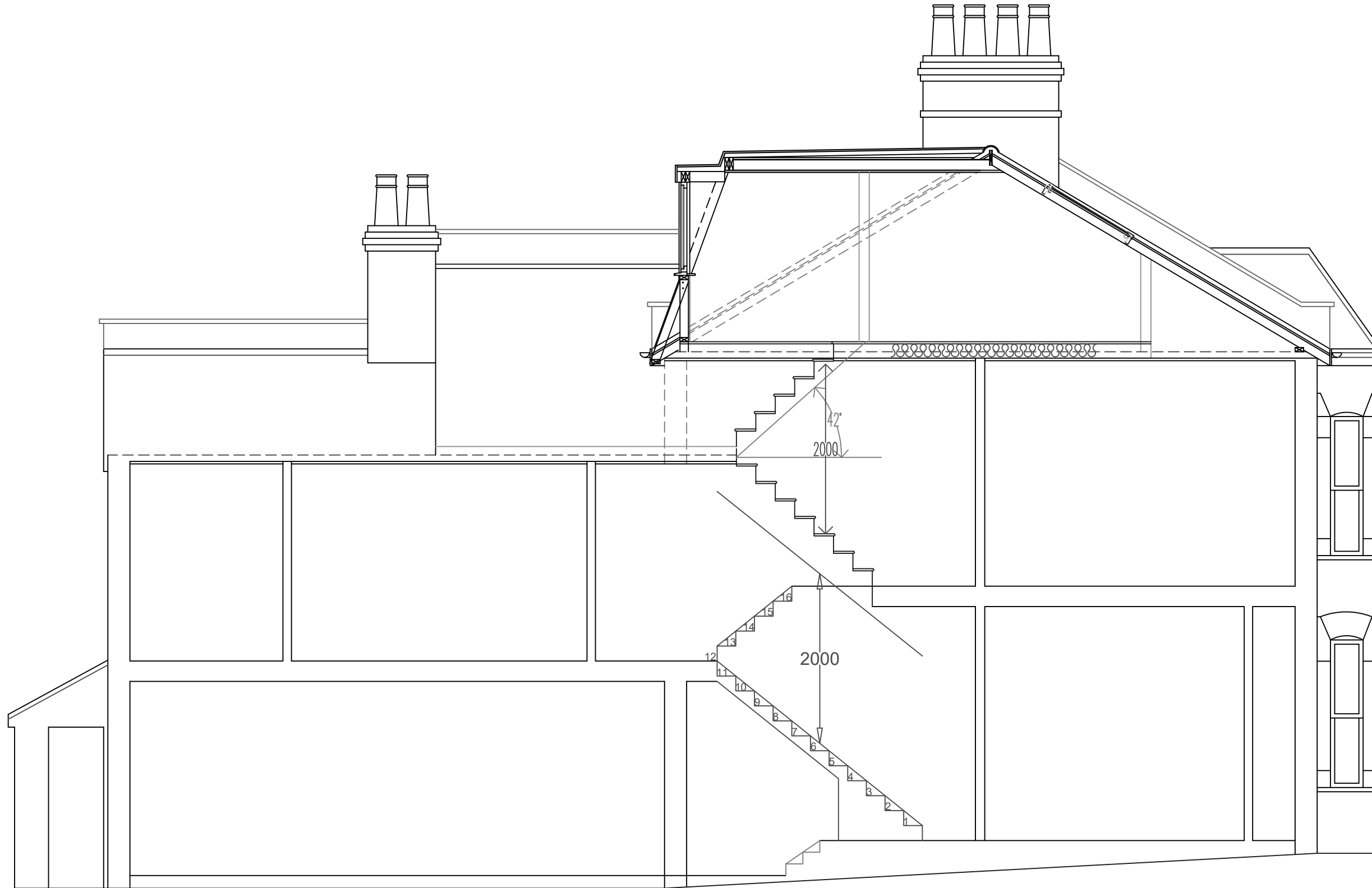
EXISTING CROSS SECTION: AA SCALE 1:50
